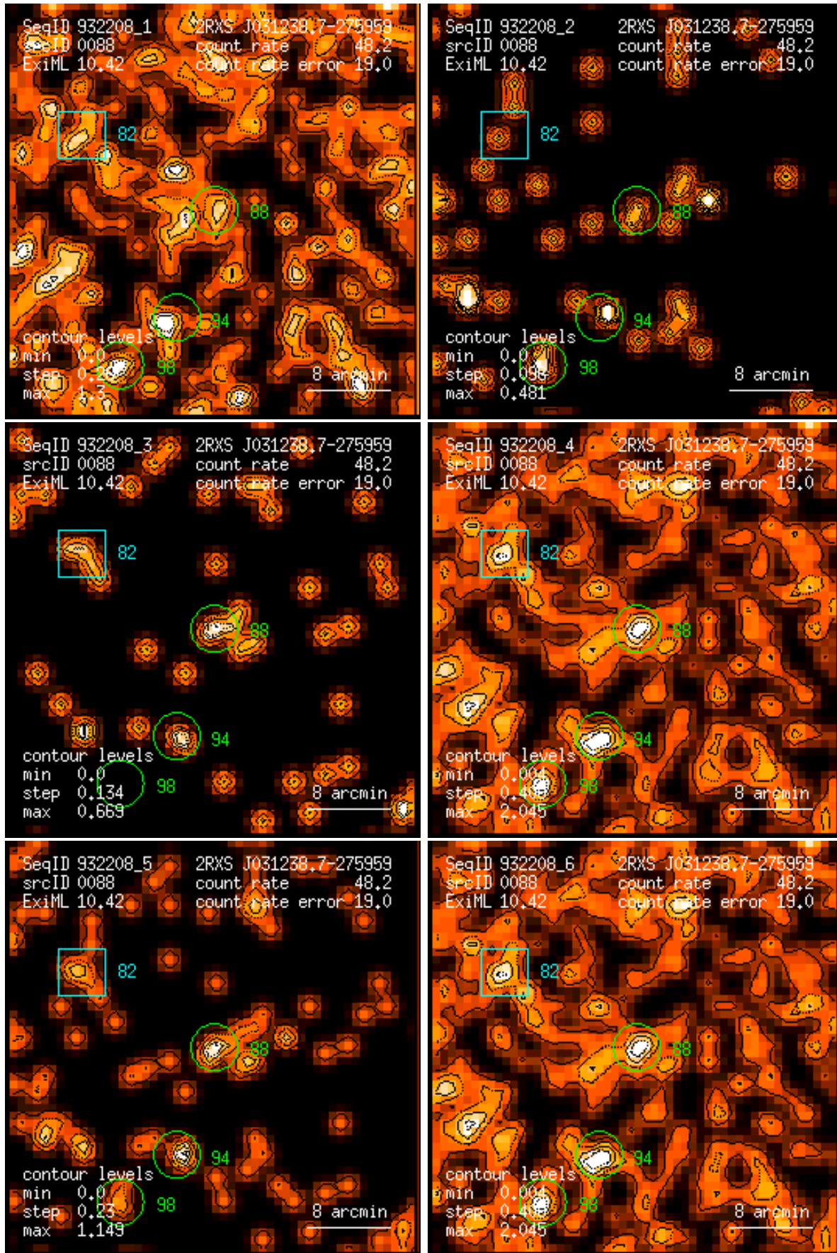
Figure 88: RASS 932208: detection 0088: band rate images, Gaussian filter: (1) PSPC channels 11 – 41, (2) 52 – 90, (3) 91 – 201, (4) 11 – 235, (5) 52 – 201, (6) 11 – 201. Broad band rates in counts/ks. Band rate contour levels in counts/ks/arcmin 2 .
