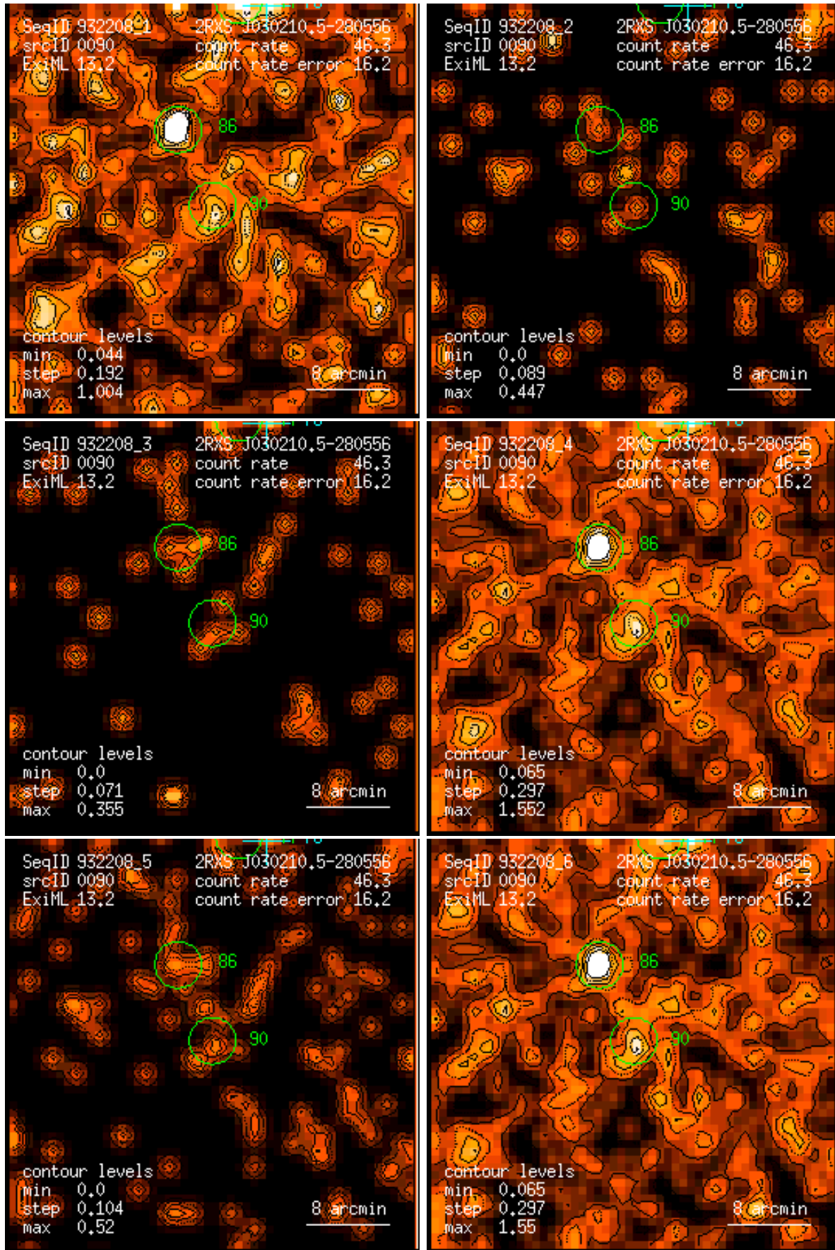
Figure 90: RASS 932208: detection 0090: band rate images, Gaussian filter: (1) PSPC channels 11 – 41, (2) 52 – 90, (3) 91 – 201, (4) 11 – 235, (5) 52 – 201, (6) 11 – 201. Broad band rates in counts/ks. Band rate contour levels in counts/ks/arcmin 2 .
