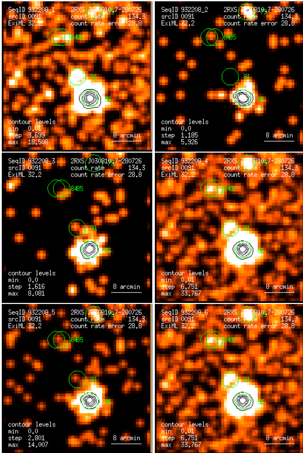
Figure 91: RASS 932208: detection 0091: band rate images, Gaussian filter: (1) PSPC channels 11 – 41, (2) 52 – 90, (3) 91 – 201, (4) 11 – 235, (5) 52 – 201, (6) 11 – 201. Broad band rates in counts/ks. Band rate contour levels in counts/ks/arcmin 2 .
