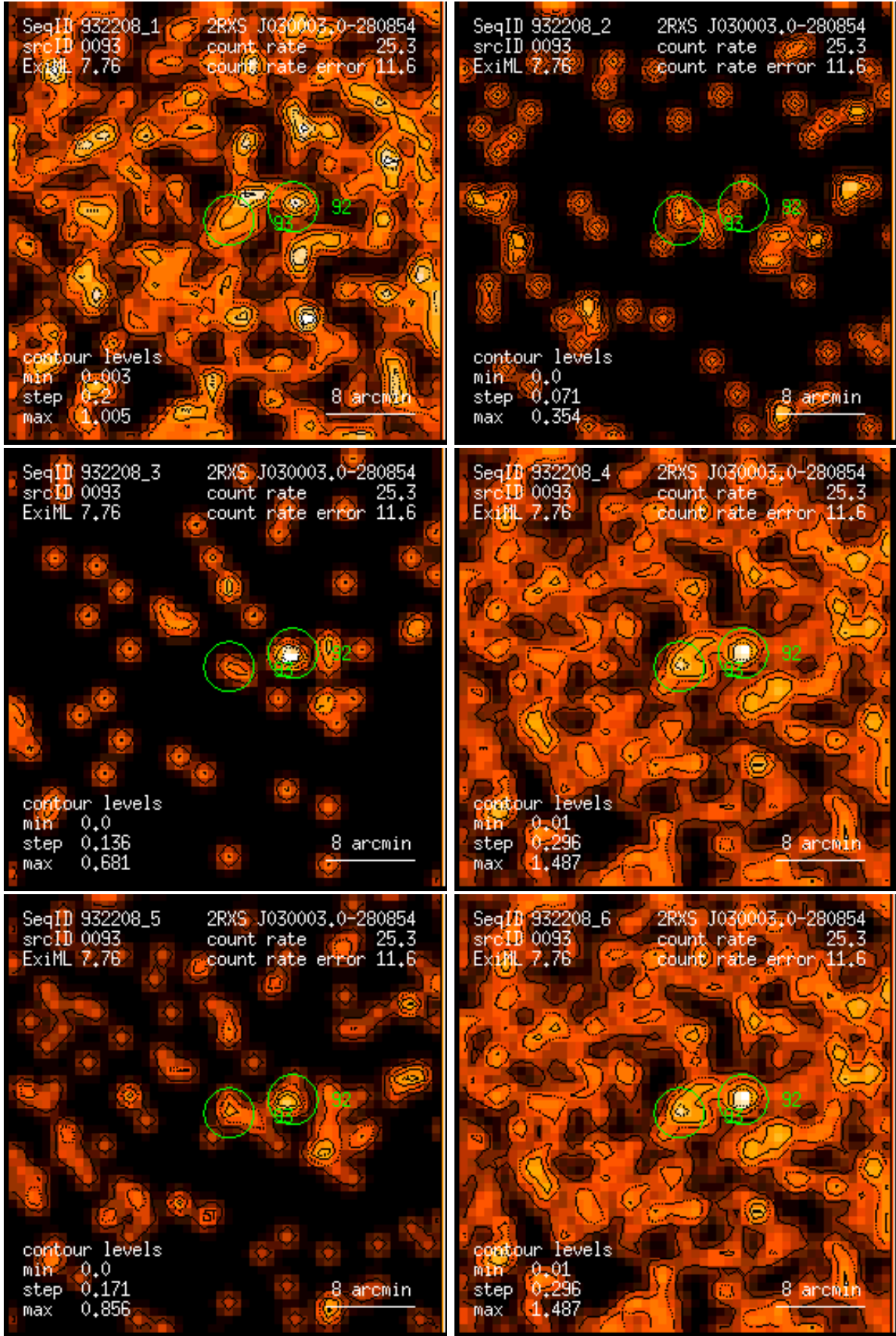
Figure 93: RASS 932208: detection 0093: band rate images, Gaussian filter: (1) PSPC channels 11 – 41, (2) 52 – 90, (3) 91 – 201, (4) 11 – 235, (5) 52 – 201, (6) 11 – 201. Broad band rates in counts/ks. Band rate contour levels in counts/ks/arcmin 2 .
