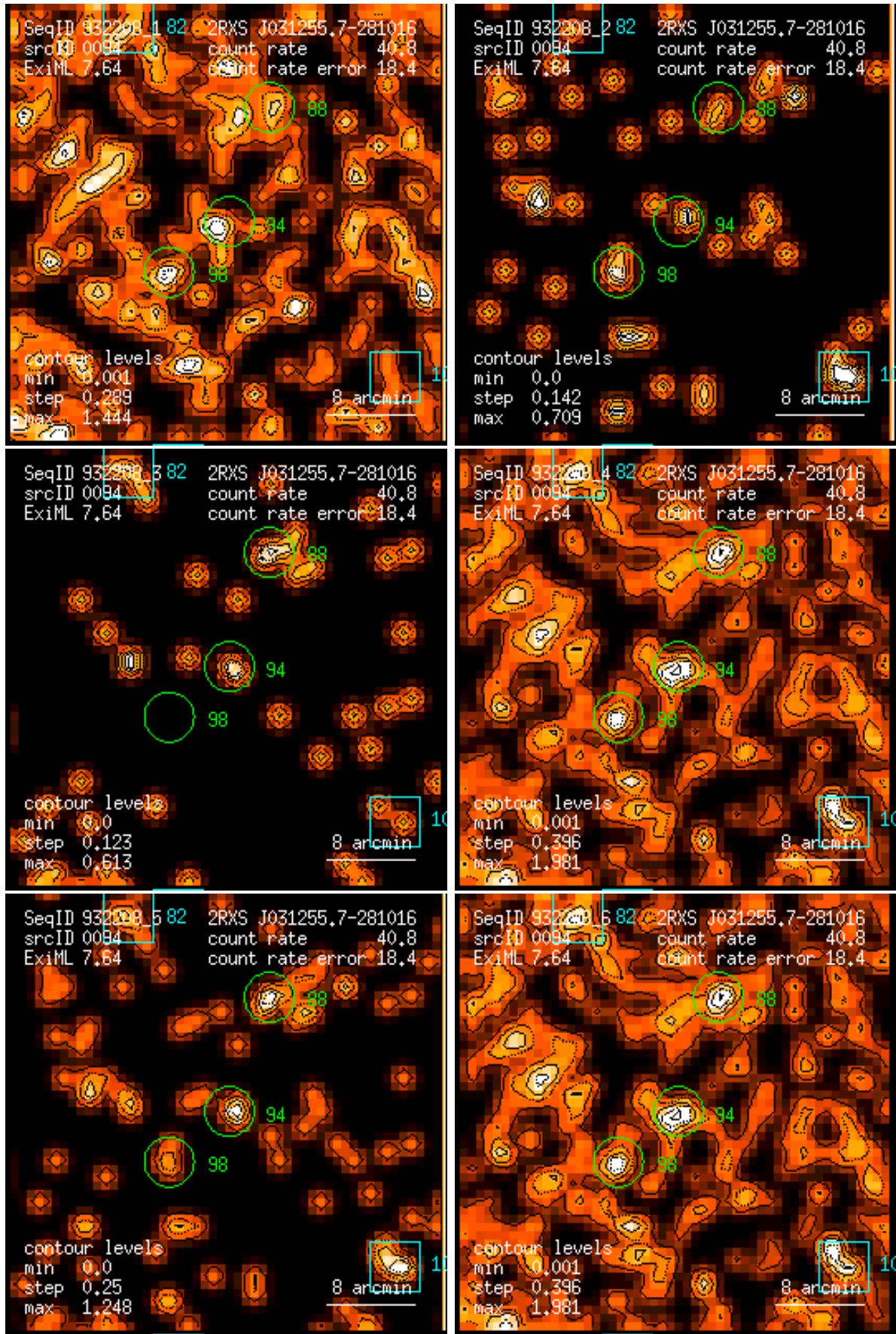
Figure 94: RASS 932208: detection 0094: band rate images, Gaussian filter: (1) PSPC channels 11 – 41, (2) 52 – 90, (3) 91 – 201, (4) 11 – 235, (5) 52 – 201, (6) 11 – 201. Broad band rates in counts/ks. Band rate contour levels in counts/ks/arcmin 2 .
