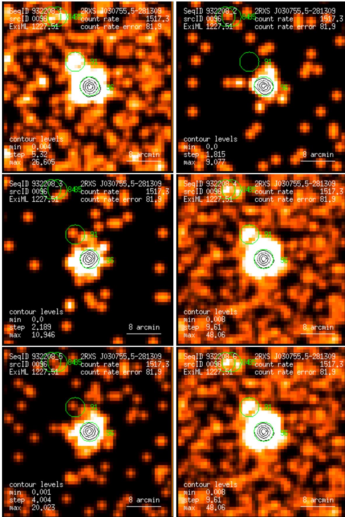
Figure 96: RASS 932208: detection 0096: band rate images, Gaussian filter: (1) PSPC channels 11 – 41, (2) 52 – 90, (3) 91 – 201, (4) 11 – 235, (5) 52 – 201, (6) 11 – 201. Broad band rates in counts/ks. Band rate contour levels in counts/ks/arcmin 2 .
