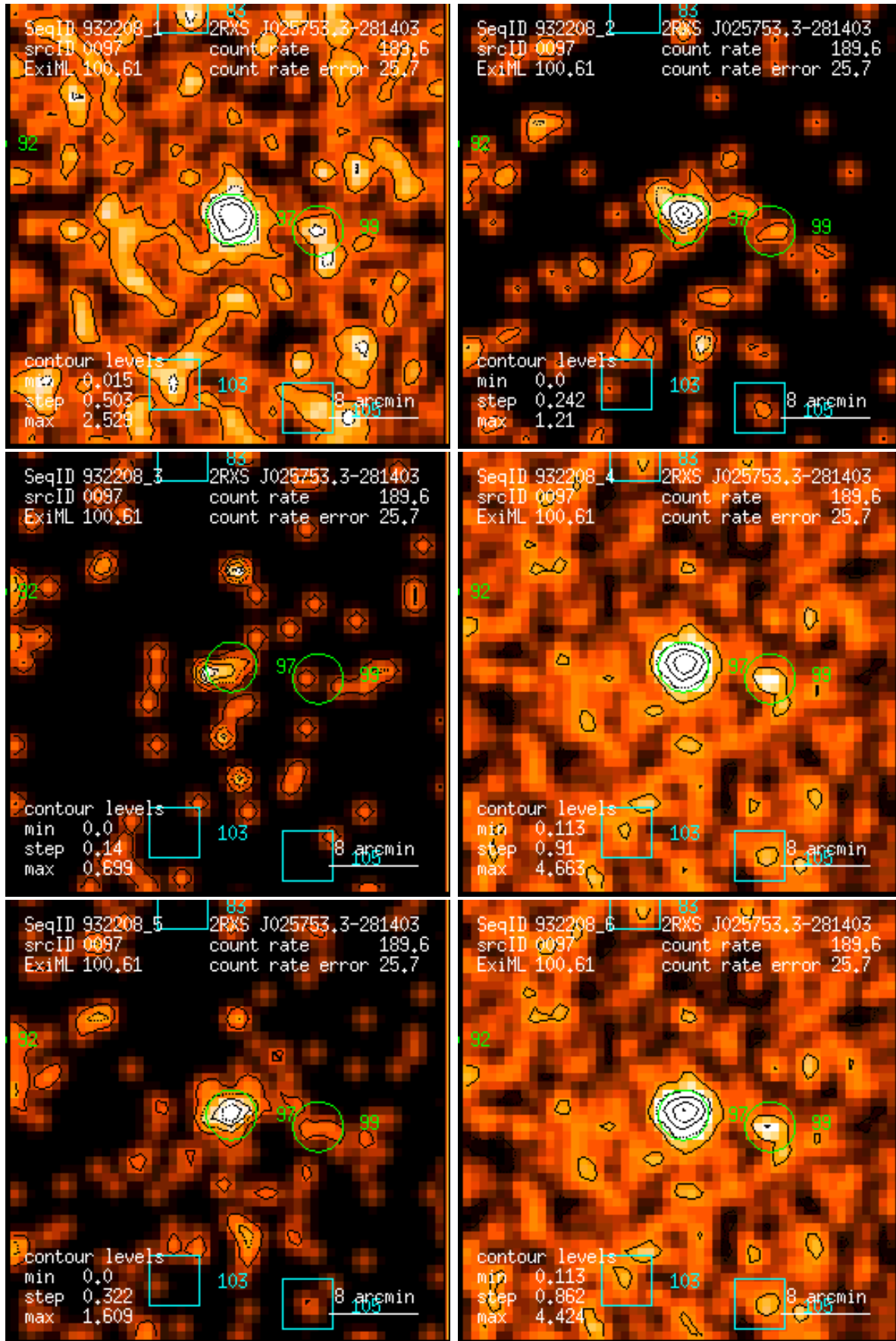
Figure 97: RASS 932208: detection 0097: band rate images, Gaussian filter: (1) PSPC channels 11 – 41, (2) 52 – 90, (3) 91 – 201, (4) 11 – 235, (5) 52 – 201, (6) 11 – 201. Broad band rates in counts/ks. Band rate contour levels in counts/ks/arcmin 2 .
