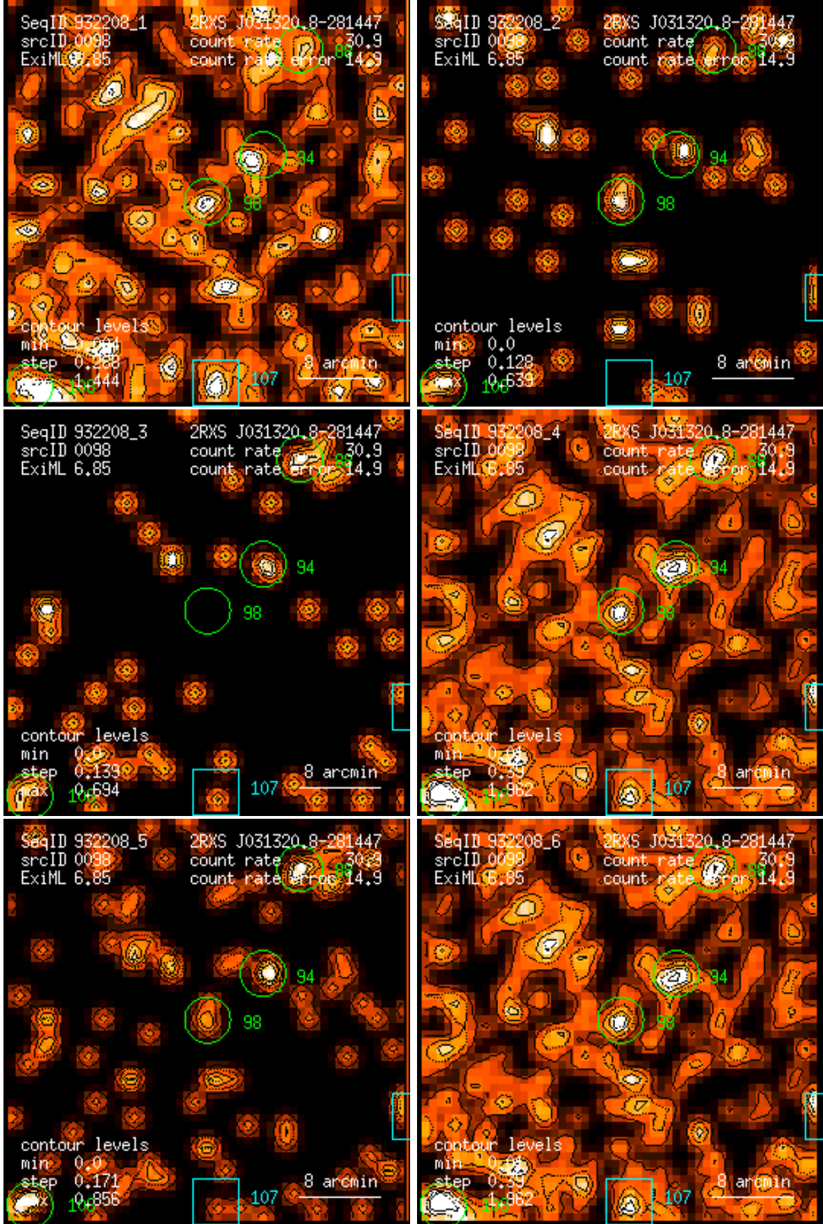
Figure 98: RASS 932208: detection 0098: band rate images, Gaussian filter: (1) PSPC channels 11 – 41, (2) 52 – 90, (3) 91 – 201, (4) 11 – 235, (5) 52 – 201, (6) 11 – 201. Broad band rates in counts/ks. Band rate contour levels in counts/ks/arcmin 2 .
