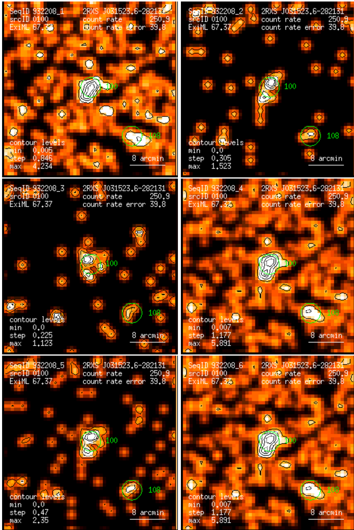
Figure 100: RASS 932208: detection 0100: band rate images, Gaussian filter: (1) PSPC channels 11 – 41, (2) 52 – 90, (3) 91 – 201, (4) 11 – 235, (5) 52 – 201, (6) 11 – 201. Broad band rates in counts/ks. Band rate contour levels in counts/ks/arcmin 2 .
