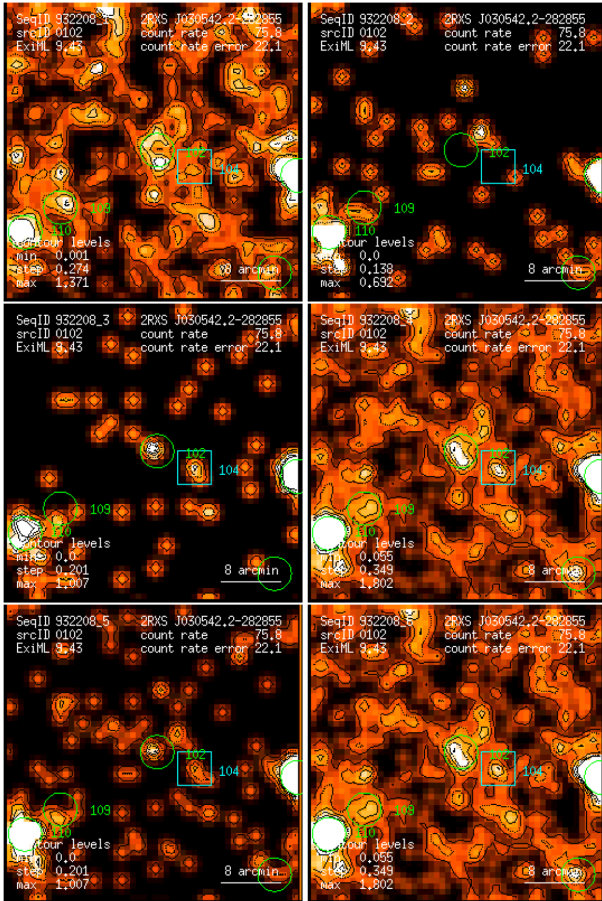
Figure 102: RASS 932208: detection 0102: band rate images, Gaussian filter: (1) PSPC channels 11 – 41, (2) 52 – 90, (3) 91 – 201, (4) 11 – 235, (5) 52 – 201, (6) 11 – 201. Broad band rates in counts/ks. Band rate contour levels in counts/ks/arcmin 2 .
