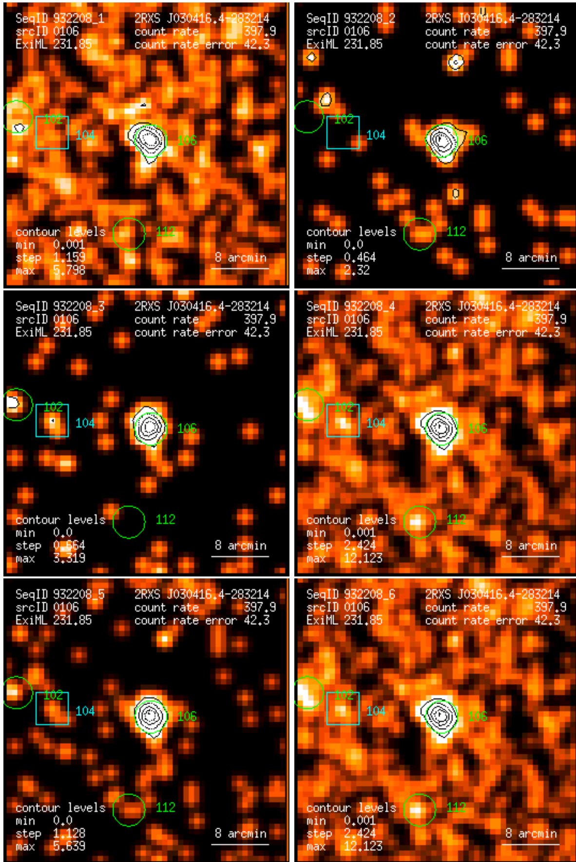
Figure 106: RASS 932208: detection 0106: band rate images, Gaussian filter: (1) PSPC channels 11 – 41, (2) 52 – 90, (3) 91 – 201, (4) 11 – 235, (5) 52 – 201, (6) 11 – 201. Broad band rates in counts/ks. Band rate contour levels in counts/ks/arcmin 2 .
