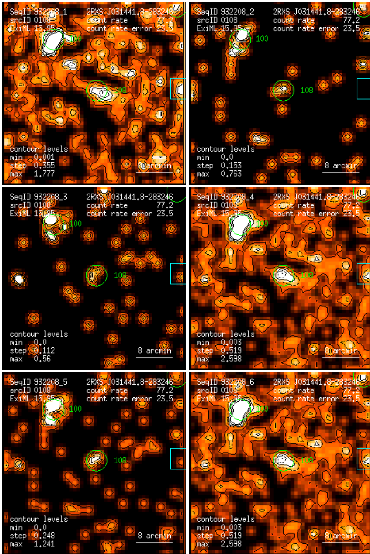
Figure 108: RASS 932208: detection 0108: band rate images, Gaussian filter: (1) PSPC channels 11 – 41, (2) 52 – 90, (3) 91 – 201, (4) 11 – 235, (5) 52 – 201, (6) 11 – 201. Broad band rates in counts/ks. Band rate contour levels in counts/ks/arcmin 2 .
