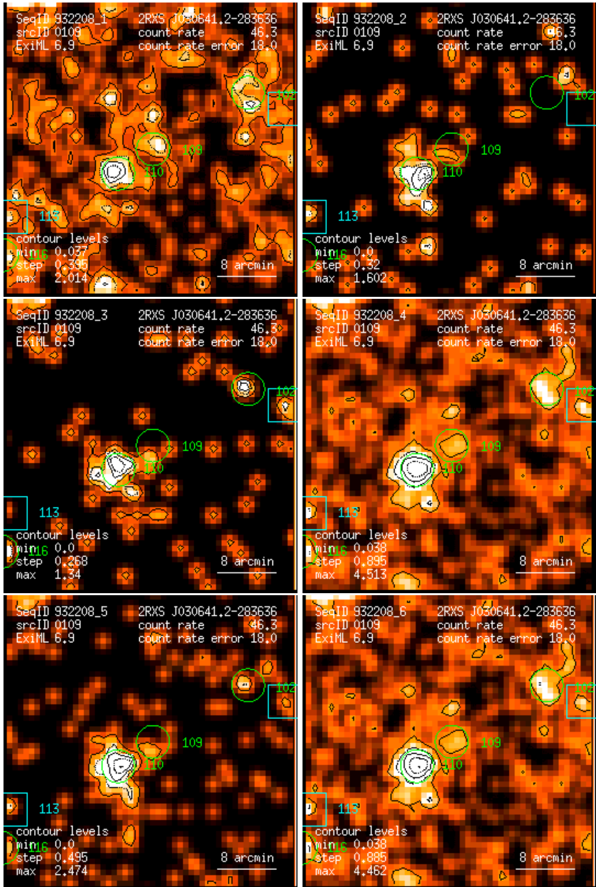
Figure 109: RASS 932208: detection 0109: band rate images, Gaussian filter: (1) PSPC channels 11 – 41, (2) 52 – 90, (3) 91 – 201, (4) 11 – 235, (5) 52 – 201, (6) 11 – 201. Broad band rates in counts/ks. Band rate contour levels in counts/ks/arcmin 2 .
