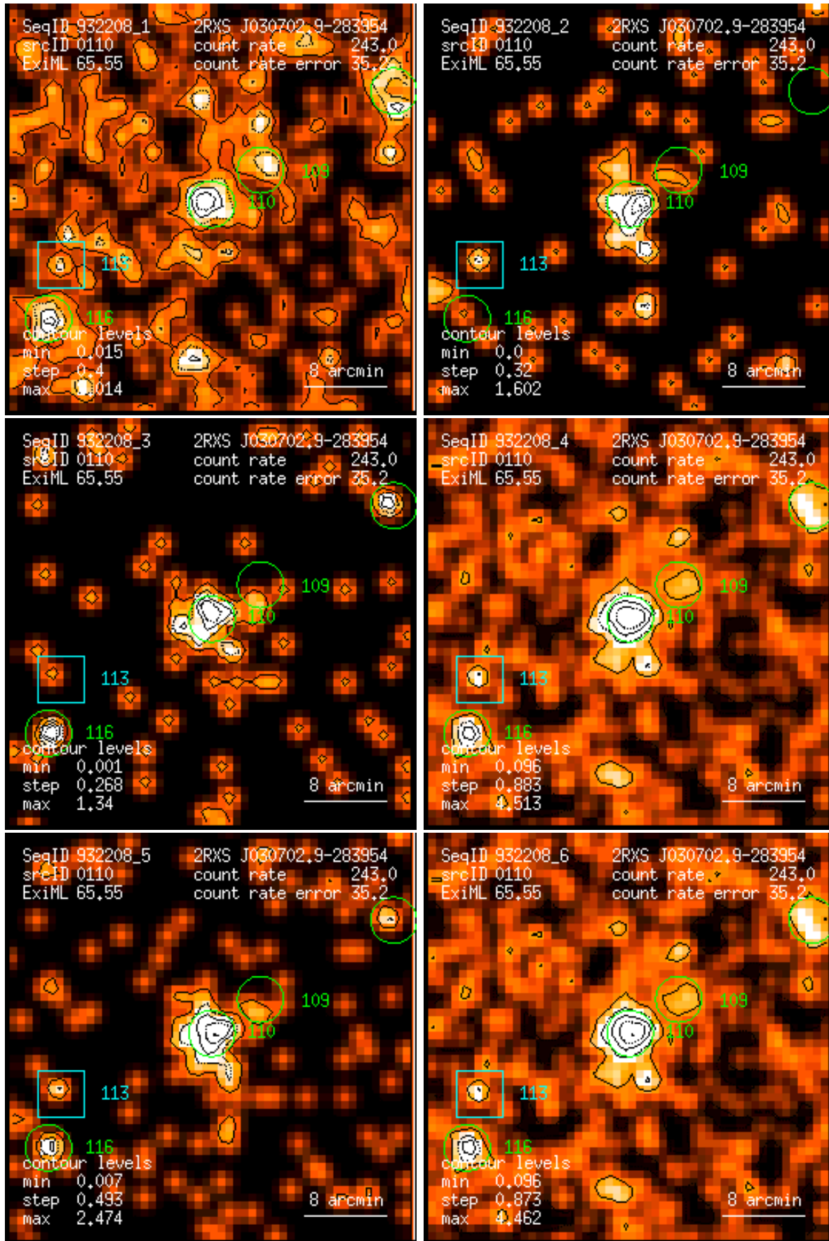
Figure 110: RASS 932208: detection 0110: band rate images, Gaussian filter: (1) PSPC channels 11 – 41, (2) 52 – 90, (3) 91 – 201, (4) 11 – 235, (5) 52 – 201, (6) 11 – 201. Broad band rates in counts/ks. Band rate contour levels in counts/ks/arcmin 2 .
