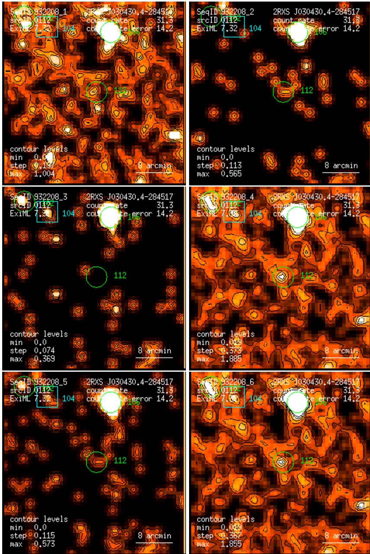
Figure 112: RASS 932208: detection 0112: band rate images, Gaussian filter: (1) PSPC channels 11 – 41, (2) 52 – 90, (3) 91 – 201, (4) 11 – 235, (5) 52 – 201, (6) 11 – 201. Broad band rates in counts/ks. Band rate contour levels in counts/ks/arcmin 2 .
