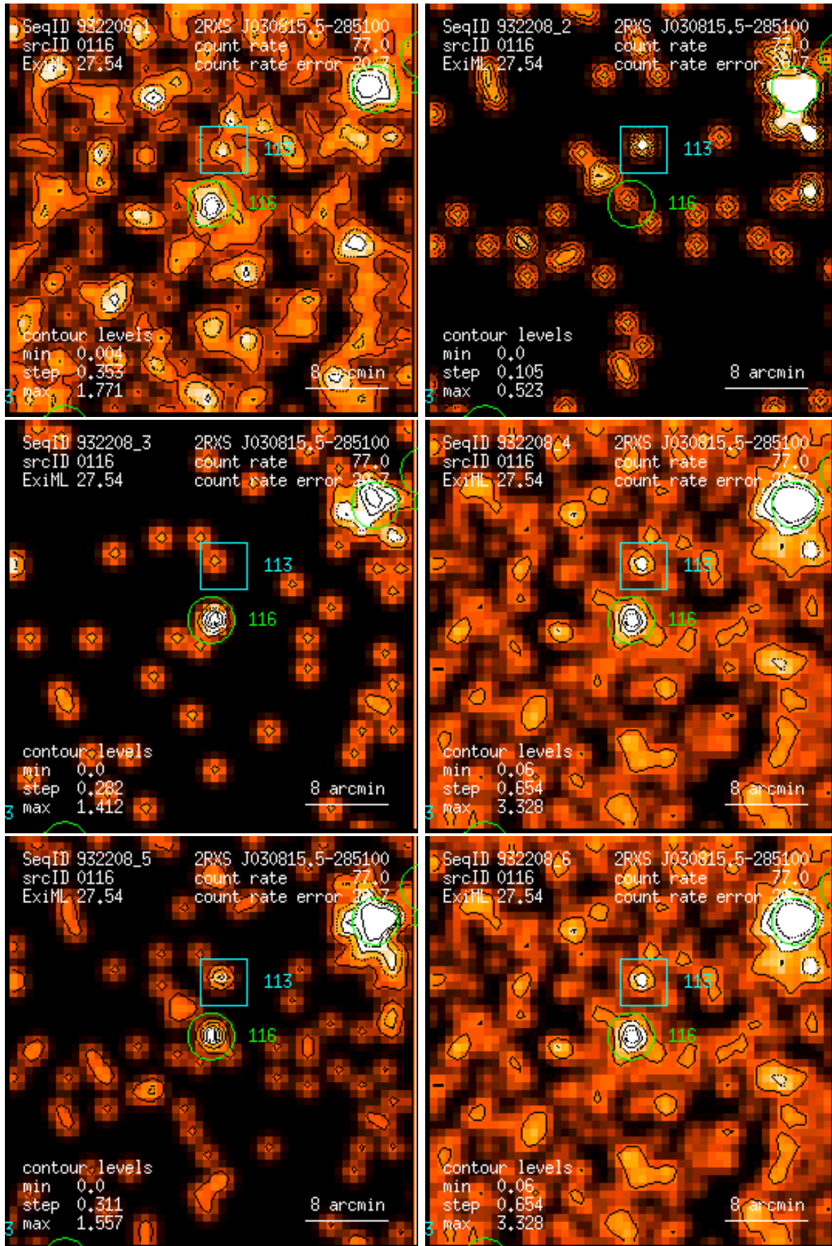
Figure 116: RASS 932208: detection 0116: band rate images, Gaussian filter: (1) PSPC channels 11 – 41, (2) 52 – 90, (3) 91 – 201, (4) 11 – 235, (5) 52 – 201, (6) 11 – 201. Broad band rates in counts/ks. Band rate contour levels in counts/ks/arcmin 2 .
