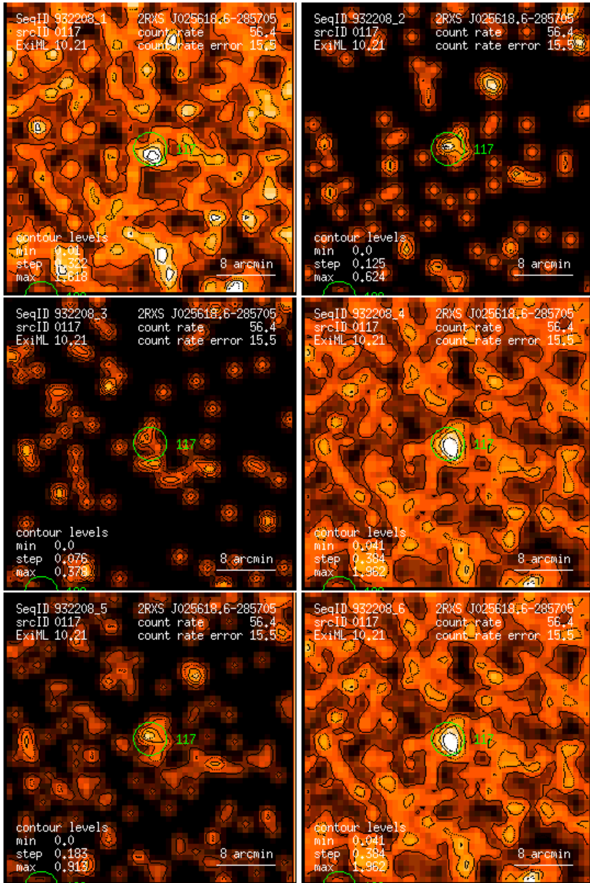
Figure 117: RASS 932208: detection 0117: band rate images, Gaussian filter: (1) PSPC channels 11 – 41, (2) 52 – 90, (3) 91 – 201, (4) 11 – 235, (5) 52 – 201, (6) 11 – 201. Broad band rates in counts/ks. Band rate contour levels in counts/ks/arcmin 2 .
