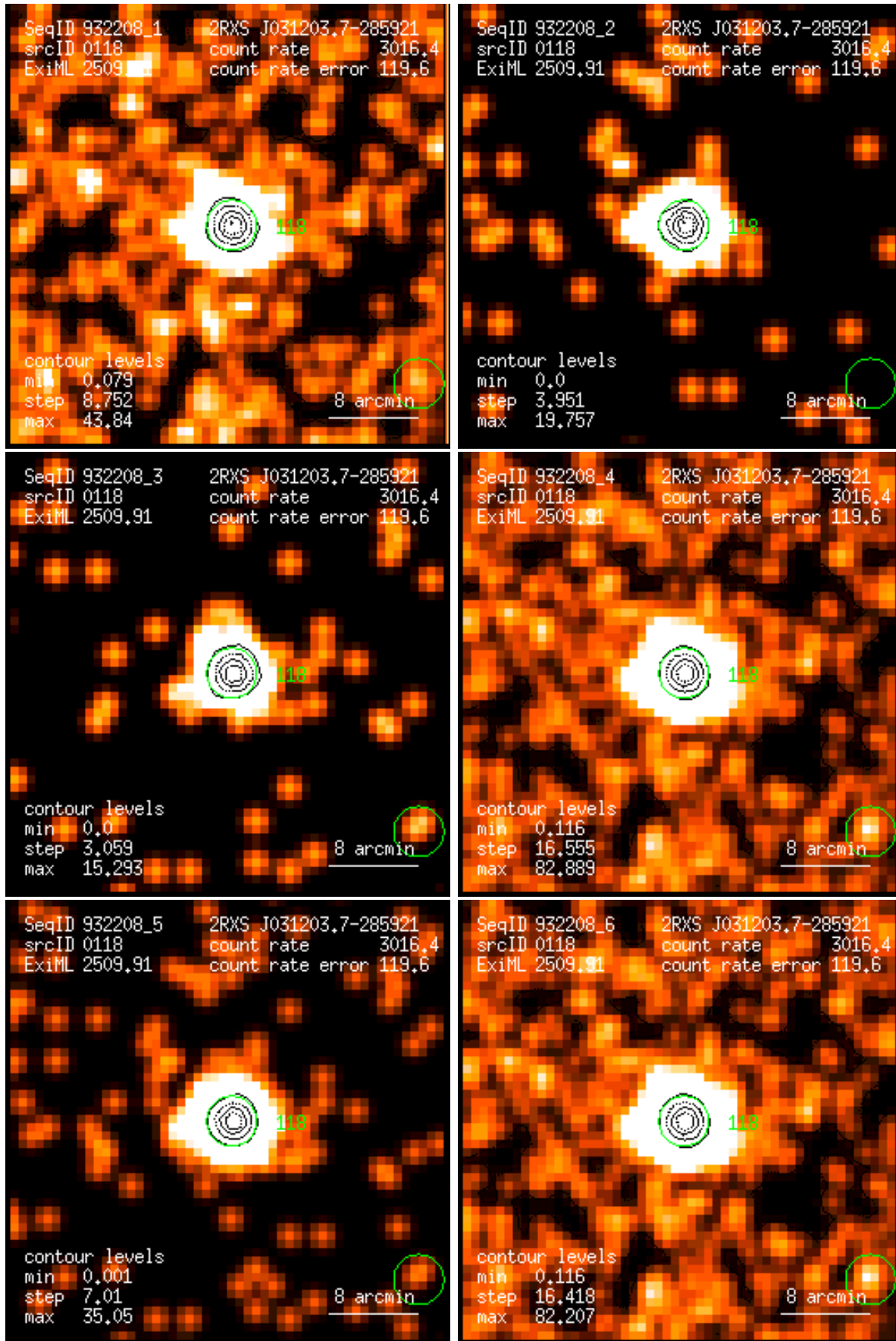
Figure 118: RASS 932208: detection 0118: band rate images, Gaussian filter: (1) PSPC channels 11 – 41, (2) 52 – 90, (3) 91 – 201, (4) 11 – 235, (5) 52 – 201, (6) 11 – 201. Broad band rates in counts/ks. Band rate contour levels in counts/ks/arcmin 2 .
