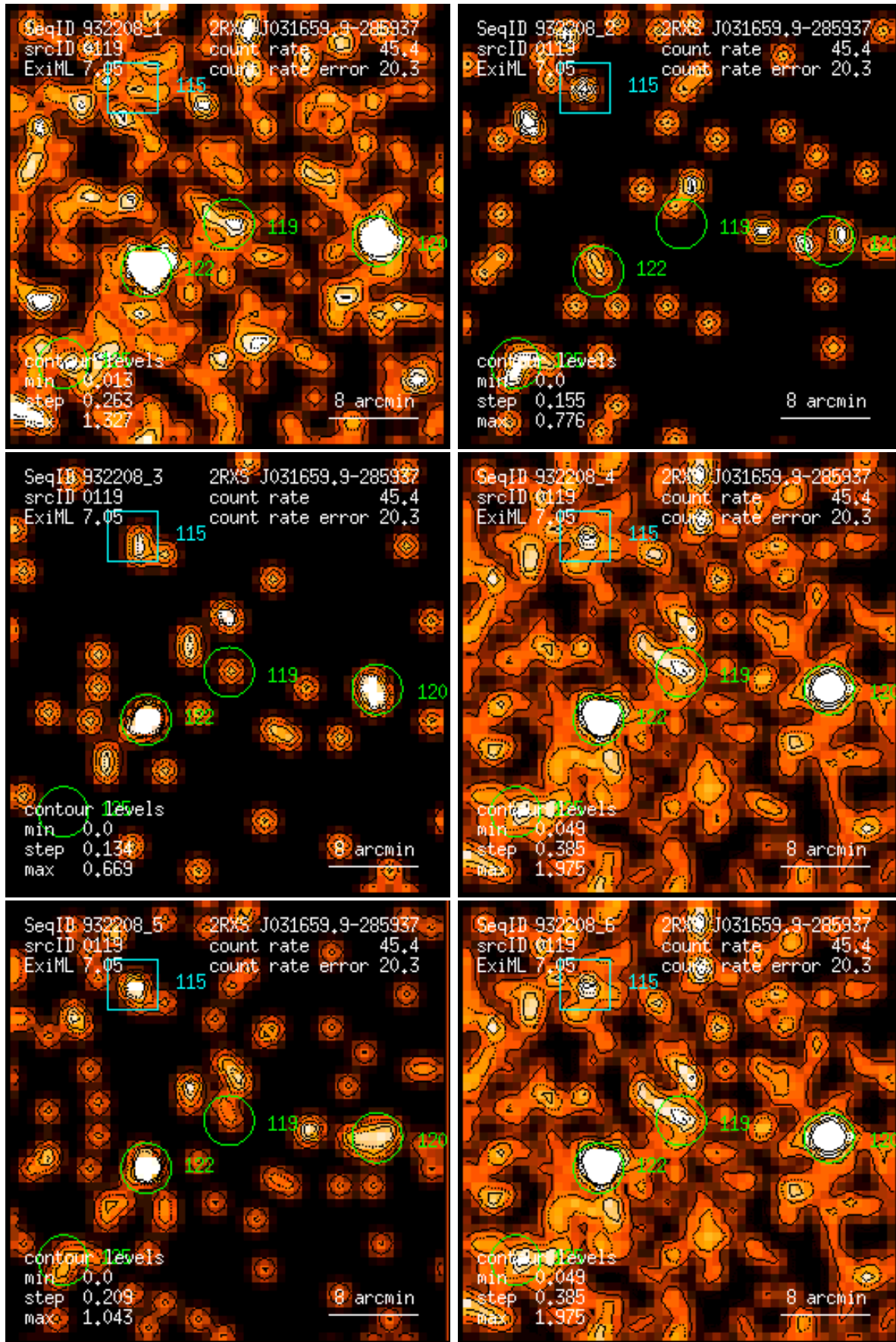
Figure 119: RASS 932208: detection 0119: band rate images, Gaussian filter: (1) PSPC channels 11 – 41, (2) 52 – 90, (3) 91 – 201, (4) 11 – 235, (5) 52 – 201, (6) 11 – 201. Broad band rates in counts/ks. Band rate contour levels in counts/ks/arcmin 2 .
