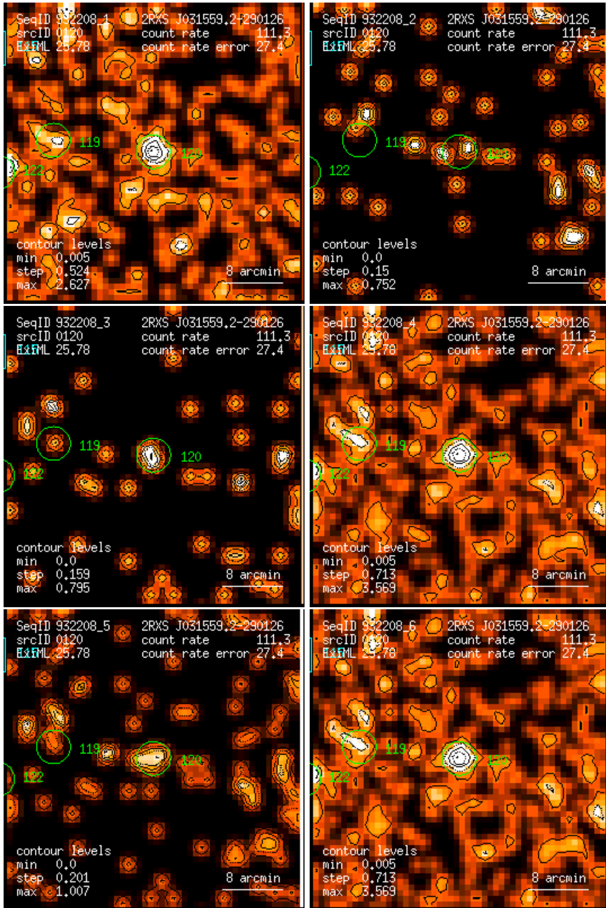
Figure 120: RASS 932208: detection 0120: band rate images, Gaussian filter: (1) PSPC channels 11 – 41, (2) 52 – 90, (3) 91 – 201, (4) 11 – 235, (5) 52 – 201, (6) 11 – 201. Broad band rates in counts/ks. Band rate contour levels in counts/ks/arcmin 2 .
