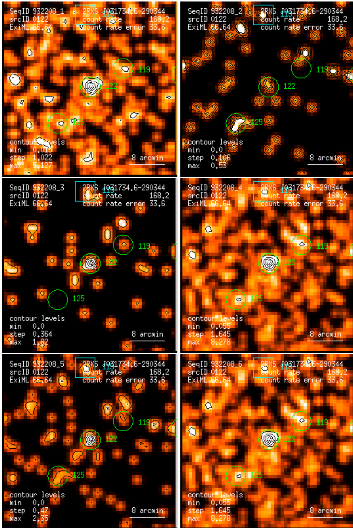
Figure 122: RASS 932208: detection 0122: band rate images, Gaussian filter: (1) PSPC channels 11 – 41, (2) 52 – 90, (3) 91 – 201, (4) 11 – 235, (5) 52 – 201, (6) 11 – 201. Broad band rates in counts/ks. Band rate contour levels in counts/ks/arcmin 2 .
