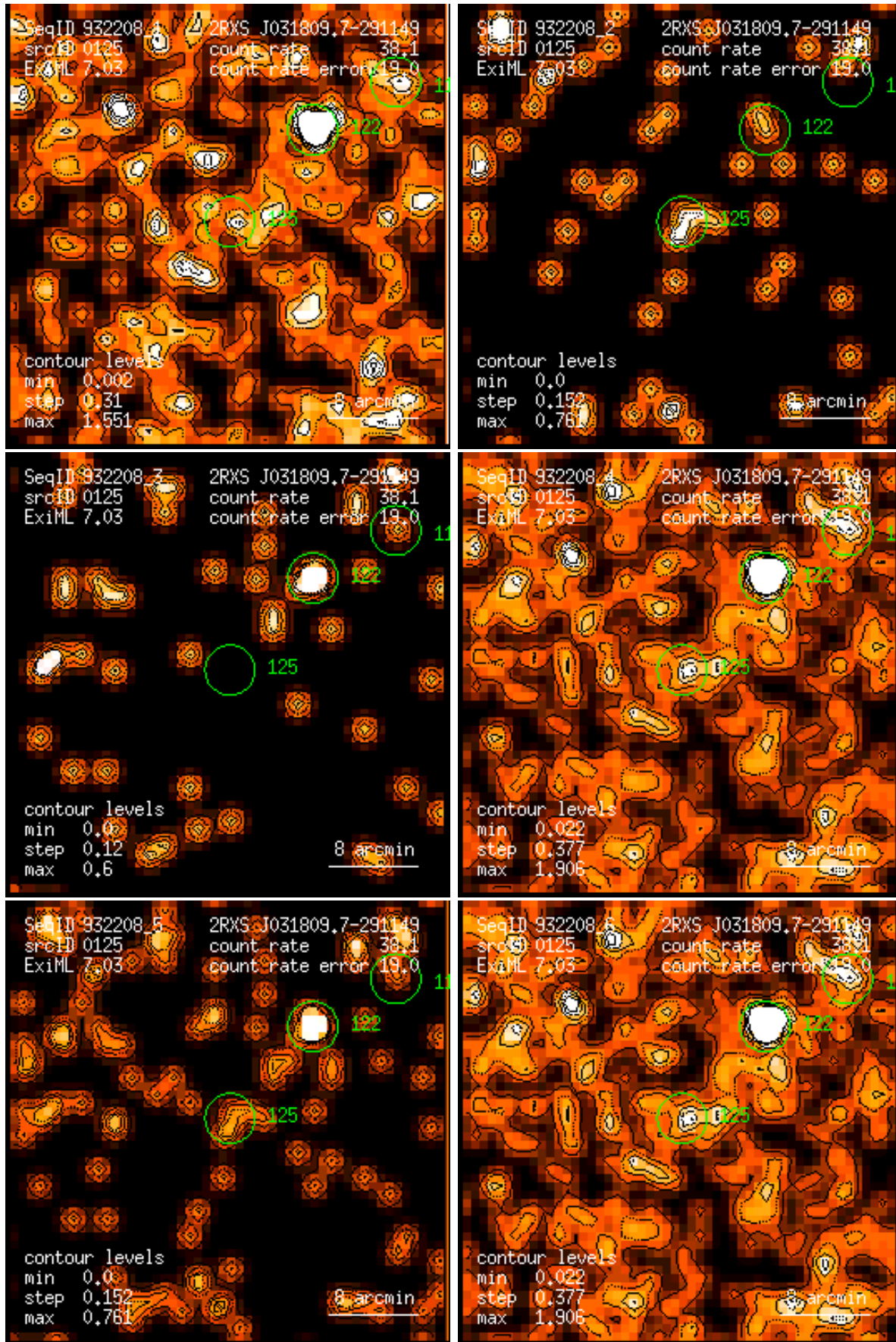
Figure 125: RASS 932208: detection 0125: band rate images, Gaussian filter: (1) PSPC channels 11 – 41, (2) 52 – 90, (3) 91 – 201, (4) 11 – 235, (5) 52 – 201, (6) 11 – 201. Broad band rates in counts/ks. Band rate contour levels in counts/ks/arcmin 2 .
