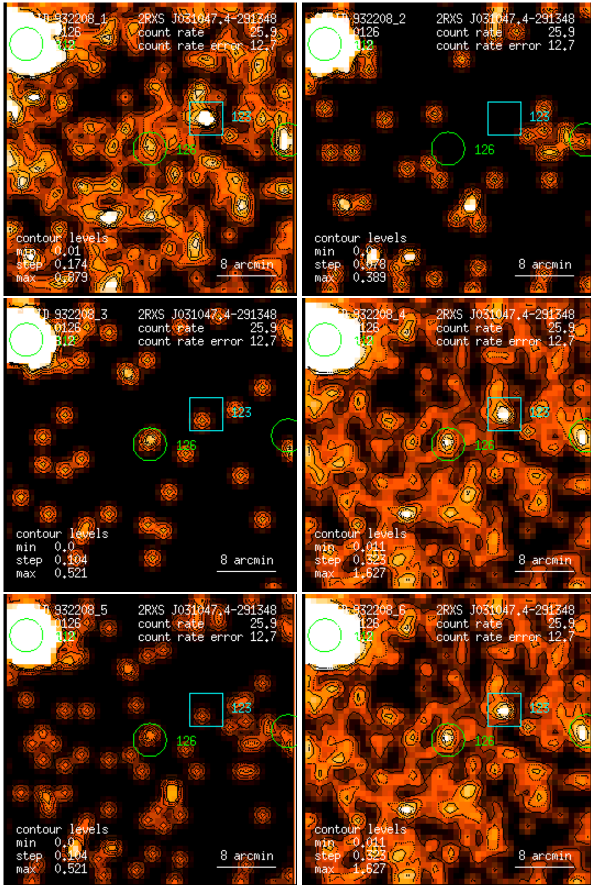
Figure 126: RASS 932208: detection 0126: band rate images, Gaussian filter: (1) PSPC channels 11 – 41, (2) 52 – 90, (3) 91 – 201, (4) 11 – 235, (5) 52 – 201, (6) 11 – 201. Broad band rates in counts/ks. Band rate contour levels in counts/ks/arcmin 2 .
