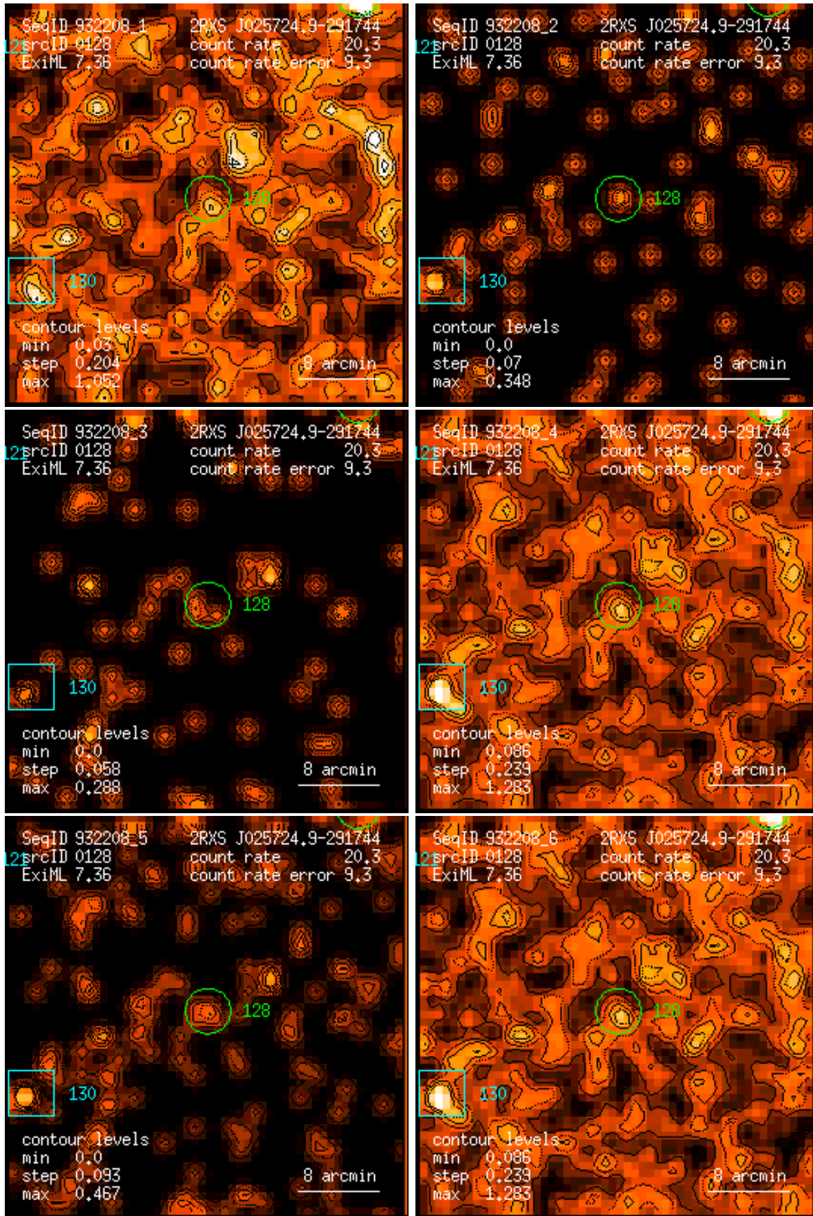
Figure 128: RASS 932208: detection 0128: band rate images, Gaussian filter: (1) PSPC channels 11 – 41, (2) 52 – 90, (3) 91 – 201, (4) 11 – 235, (5) 52 – 201, (6) 11 – 201. Broad band rates in counts/ks. Band rate contour levels in counts/ks/arcmin 2 .
