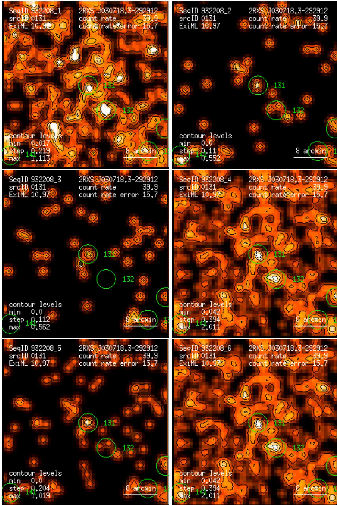
Figure 131: RASS 932208: detection 0131: band rate images, Gaussian filter: (1) PSPC channels 11 – 41, (2) 52 – 90, (3) 91 – 201, (4) 11 – 235, (5) 52 – 201, (6) 11 – 201. Broad band rates in counts/ks. Band rate contour levels in counts/ks/arcmin 2 .
