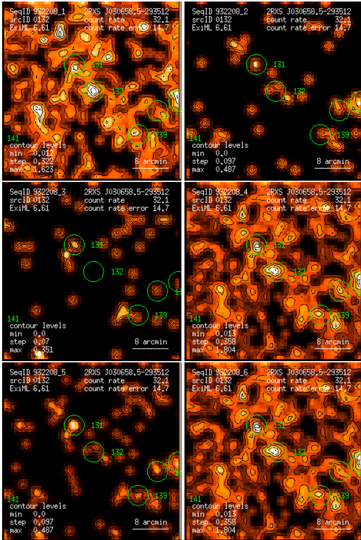
Figure 132: RASS 932208: detection 0132: band rate images, Gaussian filter: (1) PSPC channels 11 – 41, (2) 52 – 90, (3) 91 – 201, (4) 11 – 235, (5) 52 – 201, (6) 11 – 201. Broad band rates in counts/ks. Band rate contour levels in counts/ks/arcmin 2 .
