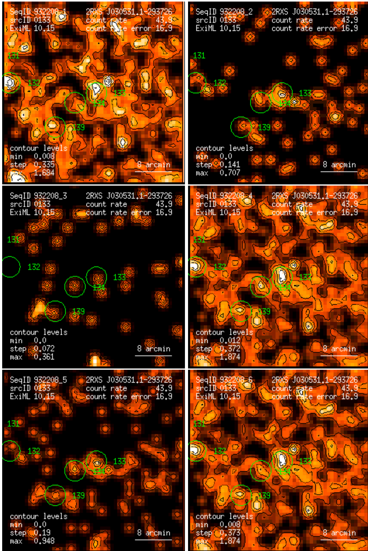
Figure 133: RASS 932208: detection 0133: band rate images, Gaussian filter: (1) PSPC channels 11 – 41, (2) 52 – 90, (3) 91 – 201, (4) 11 – 235, (5) 52 – 201, (6) 11 – 201. Broad band rates in counts/ks. Band rate contour levels in counts/ks/arcmin 2 .
