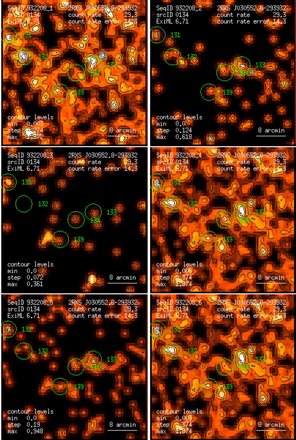
Figure 134: RASS 932208: detection 0134: band rate images, Gaussian filter: (1) PSPC channels 11 – 41, (2) 52 – 90, (3) 91 – 201, (4) 11 – 235, (5) 52 – 201, (6) 11 – 201. Broad band rates in counts/ks. Band rate contour levels in counts/ks/arcmin 2 .
