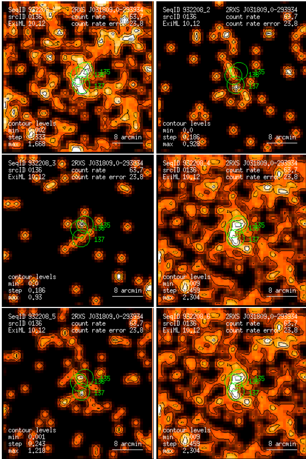
Figure 136: RASS 932208: detection 0136: band rate images, Gaussian filter: (1) PSPC channels 11 – 41, (2) 52 – 90, (3) 91 – 201, (4) 11 – 235, (5) 52 – 201, (6) 11 – 201. Broad band rates in counts/ks. Band rate contour levels in counts/ks/arcmin 2 .
