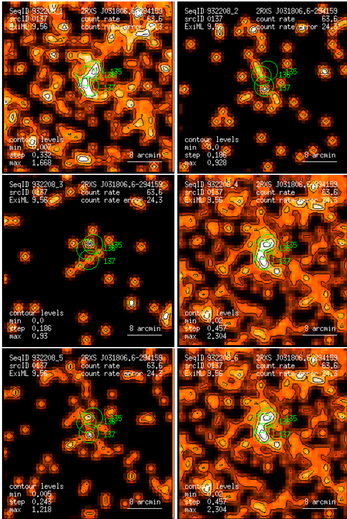
Figure 137: RASS 932208: detection 0137: band rate images, Gaussian filter: (1) PSPC channels 11 – 41, (2) 52 – 90, (3) 91 – 201, (4) 11 – 235, (5) 52 – 201, (6) 11 – 201. Broad band rates in counts/ks. Band rate contour levels in counts/ks/arcmin 2 .
