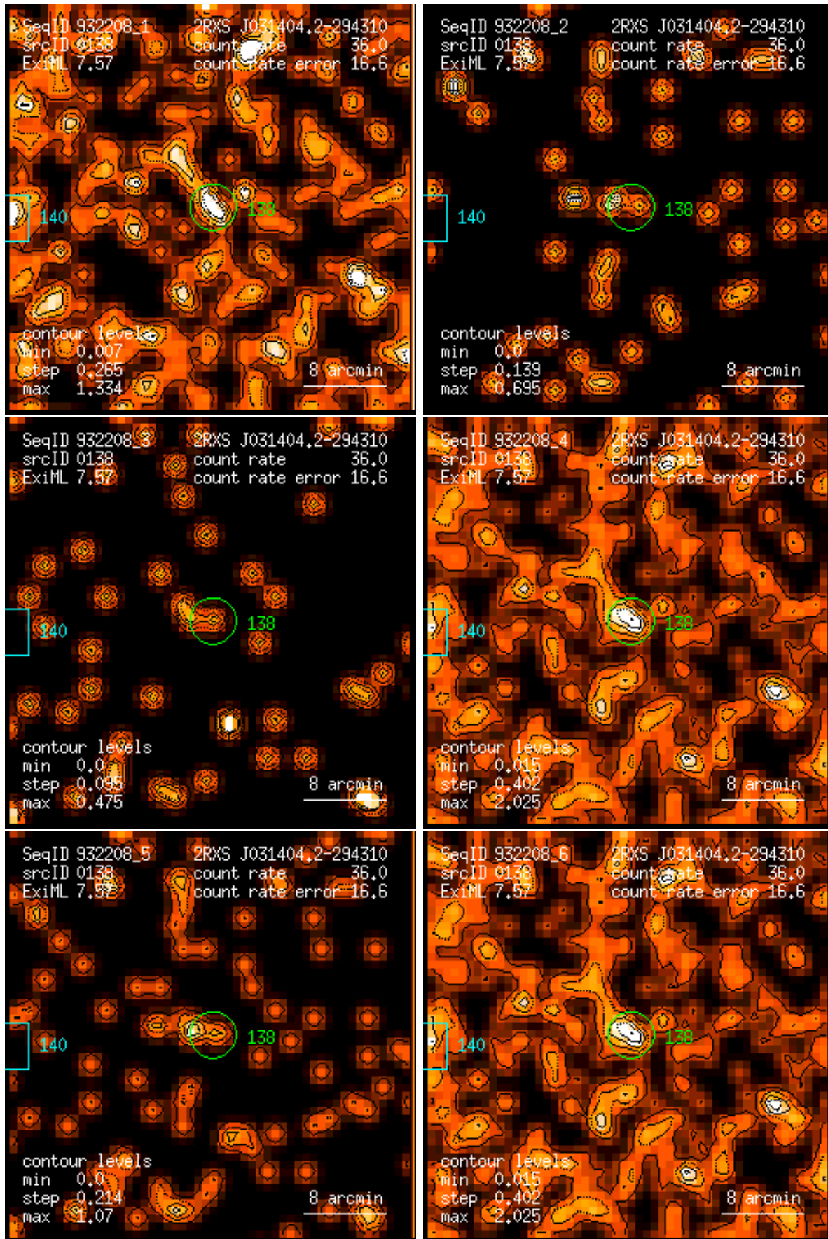
Figure 138: RASS 932208: detection 0138: band rate images, Gaussian filter: (1) PSPC channels 11 – 41, (2) 52 – 90, (3) 91 – 201, (4) 11 – 235, (5) 52 – 201, (6) 11 – 201. Broad band rates in counts/ks. Band rate contour levels in counts/ks/arcmin 2 .
