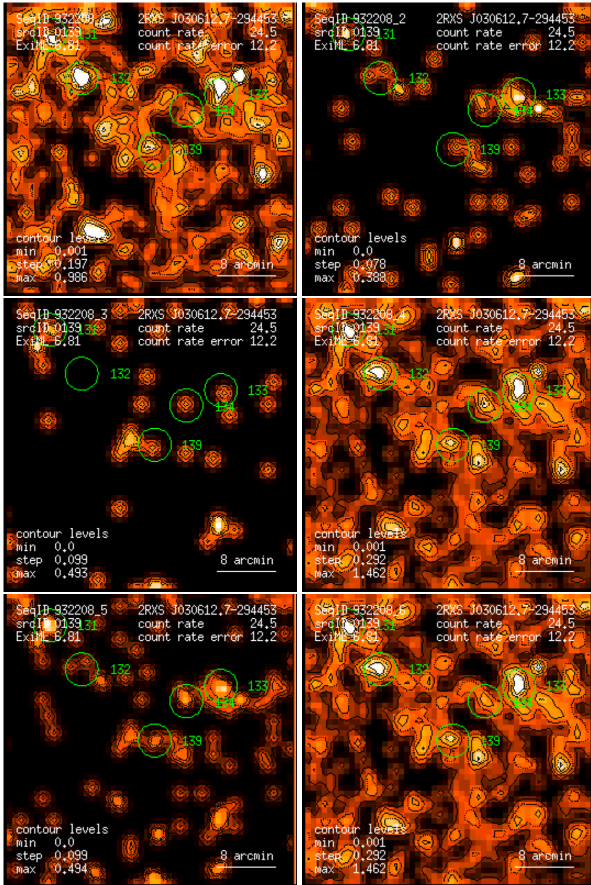
Figure 139: RASS 932208: detection 0139: band rate images, Gaussian filter: (1) PSPC channels 11 – 41, (2) 52 – 90, (3) 91 – 201, (4) 11 – 235, (5) 52 – 201, (6) 11 – 201. Broad band rates in counts/ks. Band rate contour levels in counts/ks/arcmin 2 .
