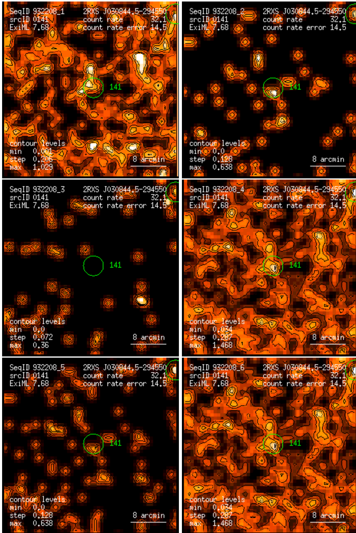
Figure 141: RASS 932208: detection 0141: band rate images, Gaussian filter: (1) PSPC channels 11 – 41, (2) 52 – 90, (3) 91 – 201, (4) 11 – 235, (5) 52 – 201, (6) 11 – 201. Broad band rates in counts/ks. Band rate contour levels in counts/ks/arcmin 2 .
