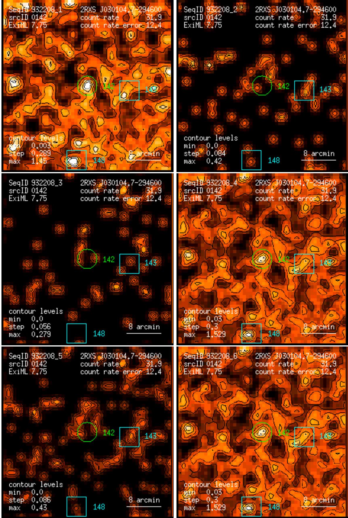
Figure 142: RASS 932208: detection 0142: band rate images, Gaussian filter: (1) PSPC channels 11 – 41, (2) 52 – 90, (3) 91 – 201, (4) 11 – 235, (5) 52 – 201, (6) 11 – 201. Broad band rates in counts/ks. Band rate contour levels in counts/ks/arcmin 2 .
