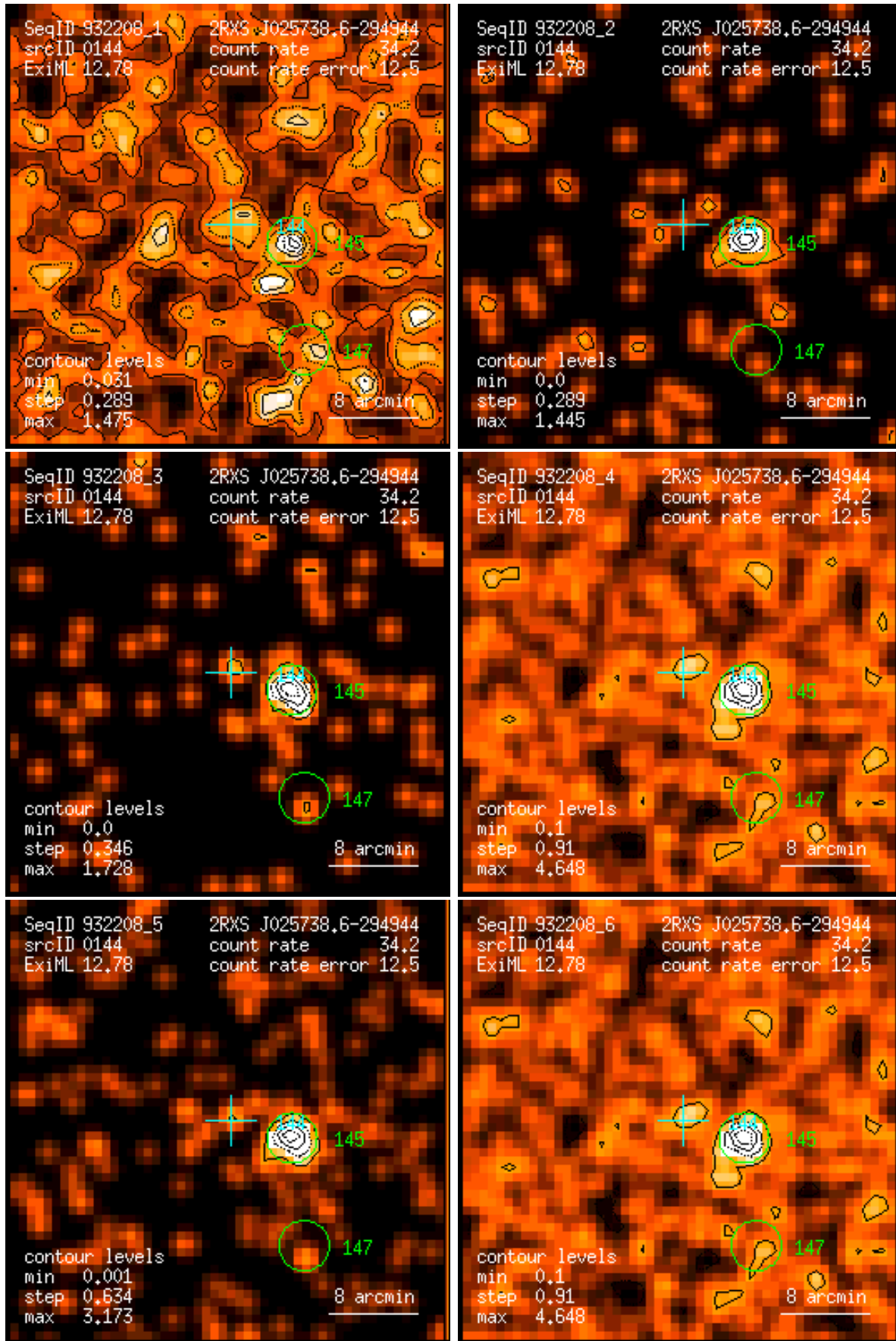
Figure 144: RASS 932208: detection 0144: band rate images, Gaussian filter: (1) PSPC channels 11 – 41, (2) 52 – 90, (3) 91 – 201, (4) 11 – 235, (5) 52 – 201, (6) 11 – 201. Broad band rates in counts/ks. Band rate contour levels in counts/ks/arcmin 2 .
