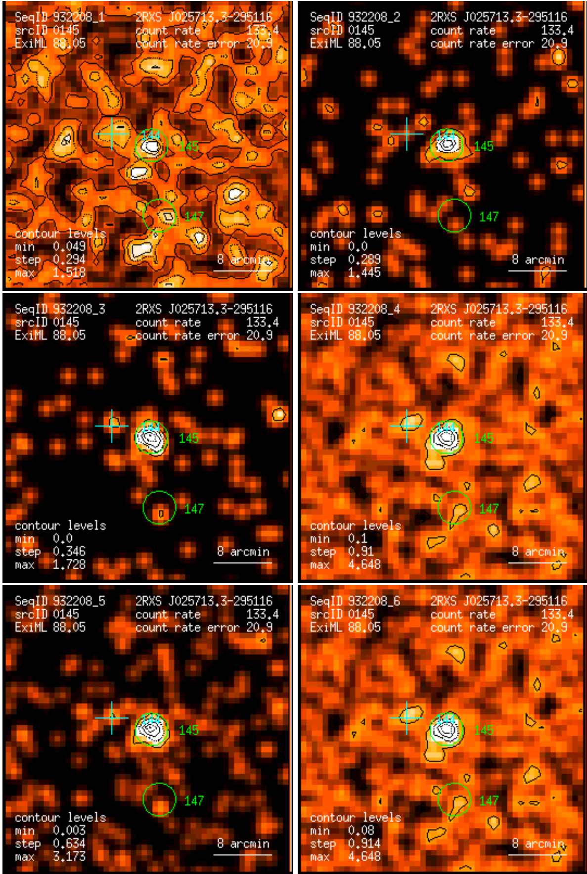
Figure 145: RASS 932208: detection 0145: band rate images, Gaussian filter: (1) PSPC channels 11 – 41, (2) 52 – 90, (3) 91 – 201, (4) 11 – 235, (5) 52 – 201, (6) 11 – 201. Broad band rates in counts/ks. Band rate contour levels in counts/ks/arcmin 2 .
