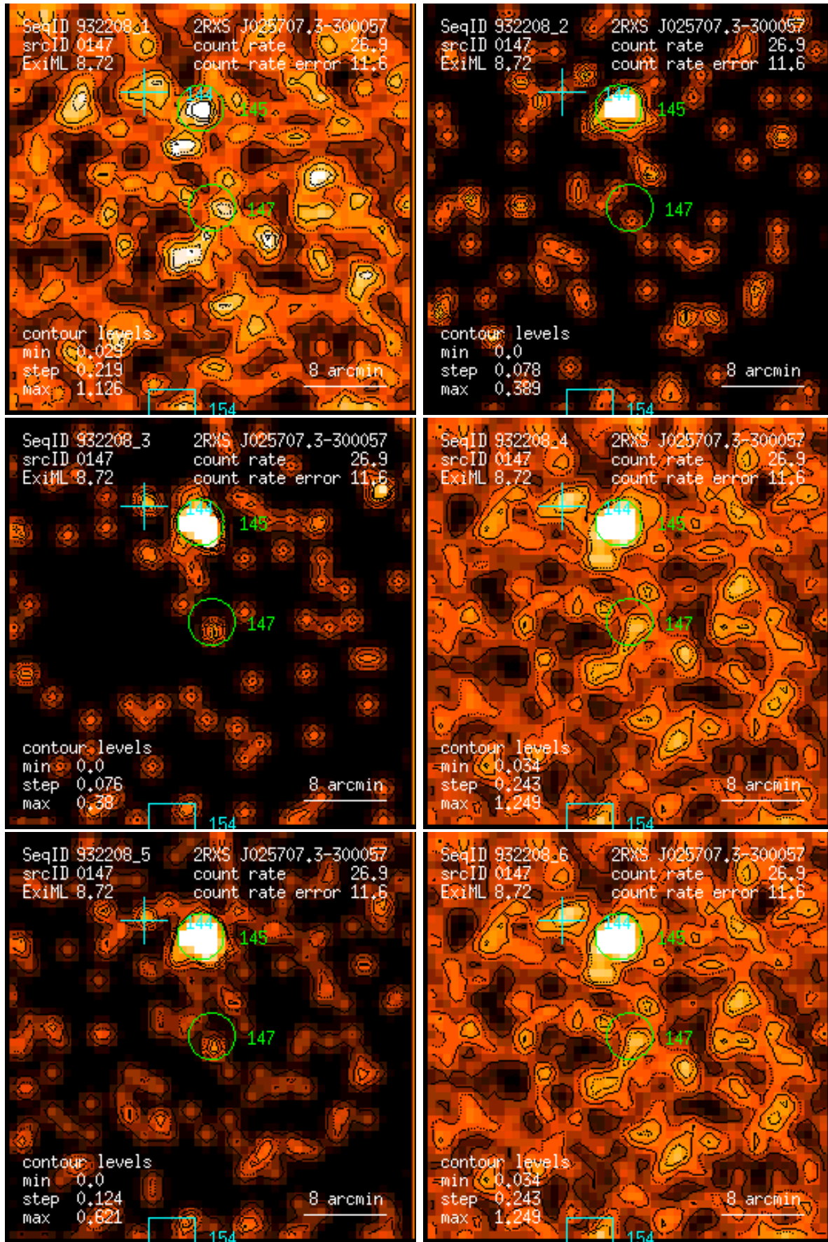
Figure 147: RASS 932208: detection 0147: band rate images, Gaussian filter: (1) PSPC channels 11 – 41, (2) 52 – 90, (3) 91 – 201, (4) 11 – 235, (5) 52 – 201, (6) 11 – 201. Broad band rates in counts/ks. Band rate contour levels in counts/ks/arcmin 2 .
