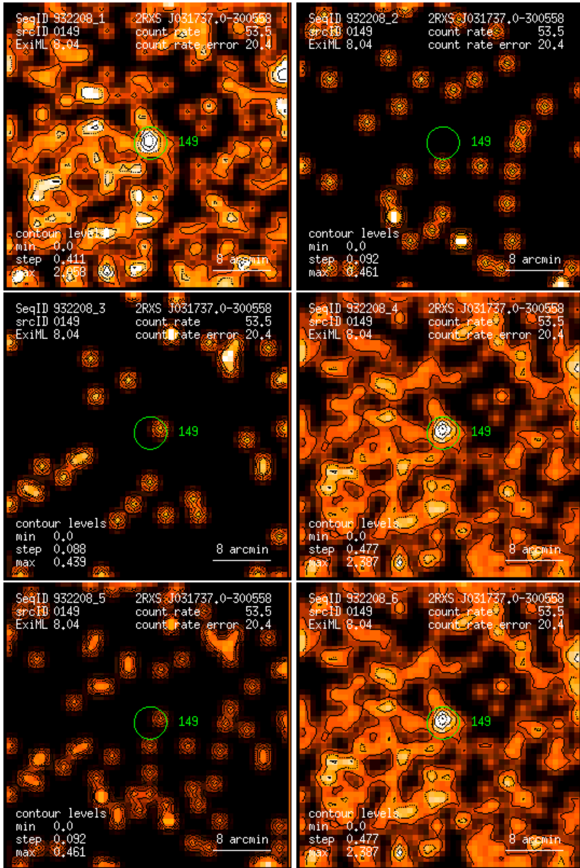
Figure 149: RASS 932208: detection 0149: band rate images, Gaussian filter: (1) PSPC channels 11 – 41, (2) 52 – 90, (3) 91 – 201, (4) 11 – 235, (5) 52 – 201, (6) 11 – 201. Broad band rates in counts/ks. Band rate contour levels in counts/ks/arcmin 2 .
