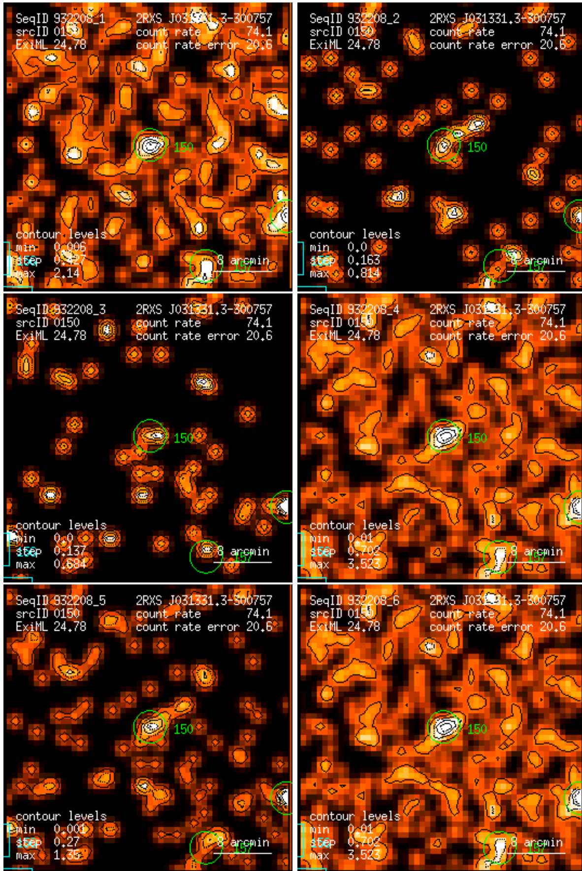
Figure 150: RASS 932208: detection 0150: band rate images, Gaussian filter: (1) PSPC channels 11 – 41, (2) 52 – 90, (3) 91 – 201, (4) 11 – 235, (5) 52 – 201, (6) 11 – 201. Broad band rates in counts/ks. Band rate contour levels in counts/ks/arcmin 2 .
