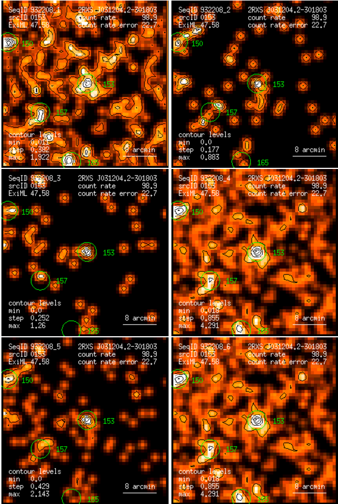
Figure 153: RASS 932208: detection 0153: band rate images, Gaussian filter: (1) PSPC channels 11 – 41, (2) 52 – 90, (3) 91 – 201, (4) 11 – 235, (5) 52 – 201, (6) 11 – 201. Broad band rates in counts/ks. Band rate contour levels in counts/ks/arcmin 2 .
