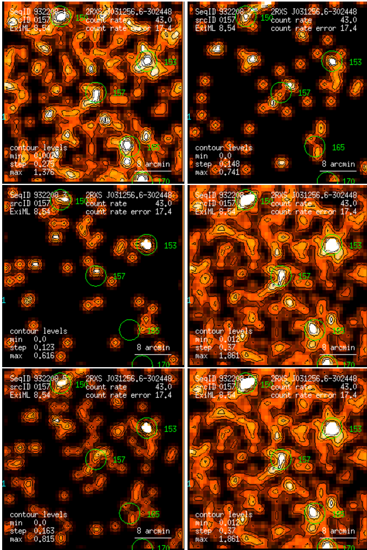
Figure 157: RASS 932208: detection 0157: band rate images, Gaussian filter: (1) PSPC channels 11 – 41, (2) 52 – 90, (3) 91 – 201, (4) 11 – 235, (5) 52 – 201, (6) 11 – 201. Broad band rates in counts/ks. Band rate contour levels in counts/ks/arcmin 2 .
