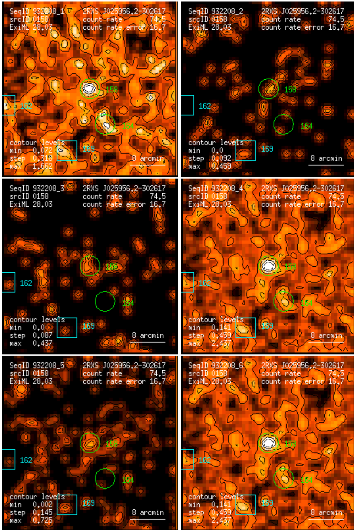
Figure 158: RASS 932208: detection 0158: band rate images, Gaussian filter: (1) PSPC channels 11 – 41, (2) 52 – 90, (3) 91 – 201, (4) 11 – 235, (5) 52 – 201, (6) 11 – 201. Broad band rates in counts/ks. Band rate contour levels in counts/ks/arcmin 2 .
