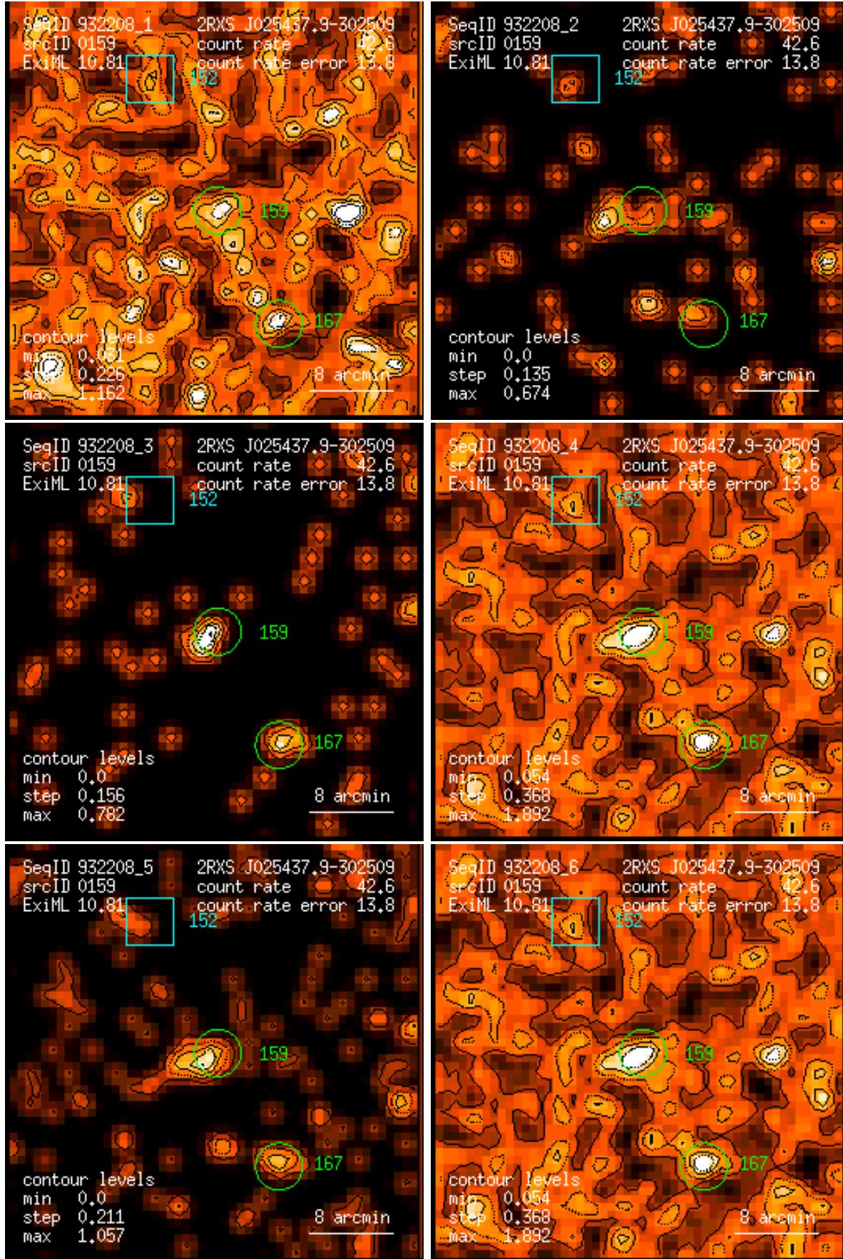
Figure 159: RASS 932208: detection 0159: band rate images, Gaussian filter: (1) PSPC channels 11 – 41, (2) 52 – 90, (3) 91 – 201, (4) 11 – 235, (5) 52 – 201, (6) 11 – 201. Broad band rates in counts/ks. Band rate contour levels in counts/ks/arcmin 2 .
