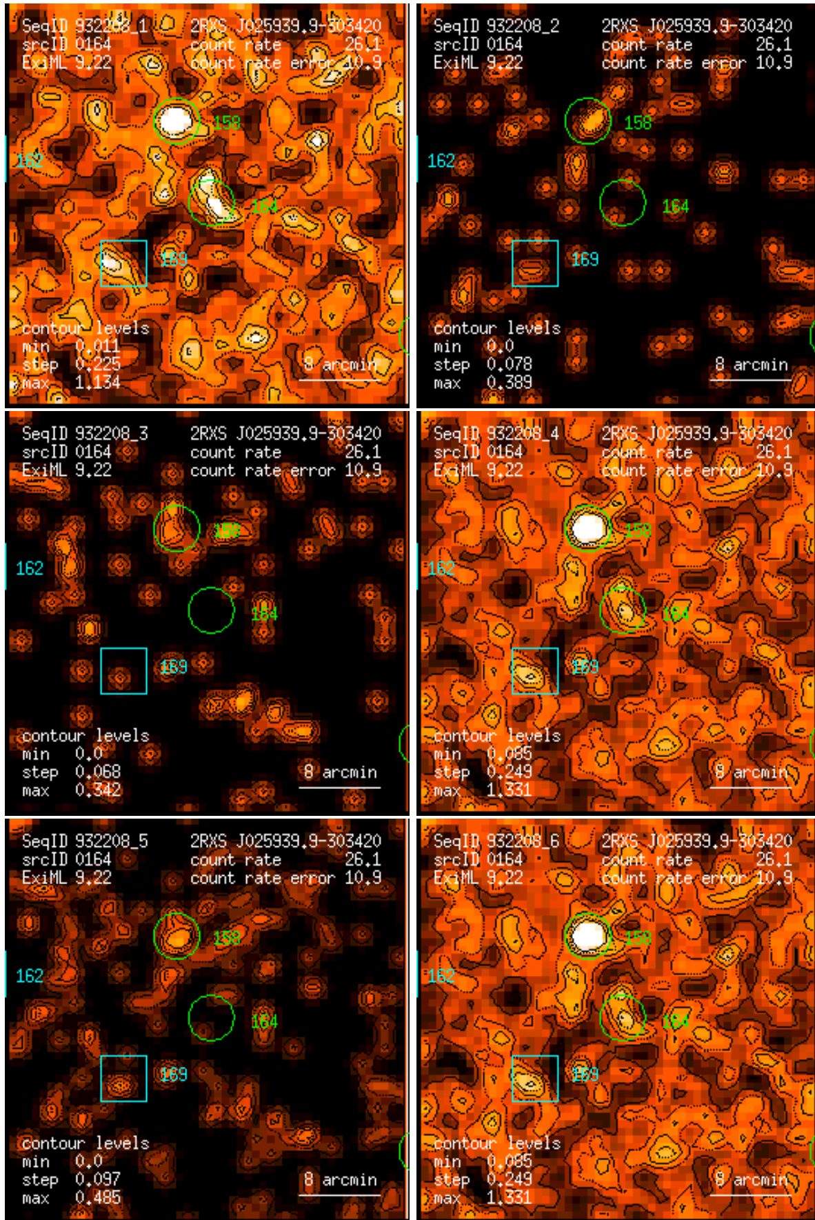
Figure 164: RASS 932208: detection 0164: band rate images, Gaussian filter: (1) PSPC channels 11 – 41, (2) 52 – 90, (3) 91 – 201, (4) 11 – 235, (5) 52 – 201, (6) 11 – 201. Broad band rates in counts/ks. Band rate contour levels in counts/ks/arcmin 2 .
