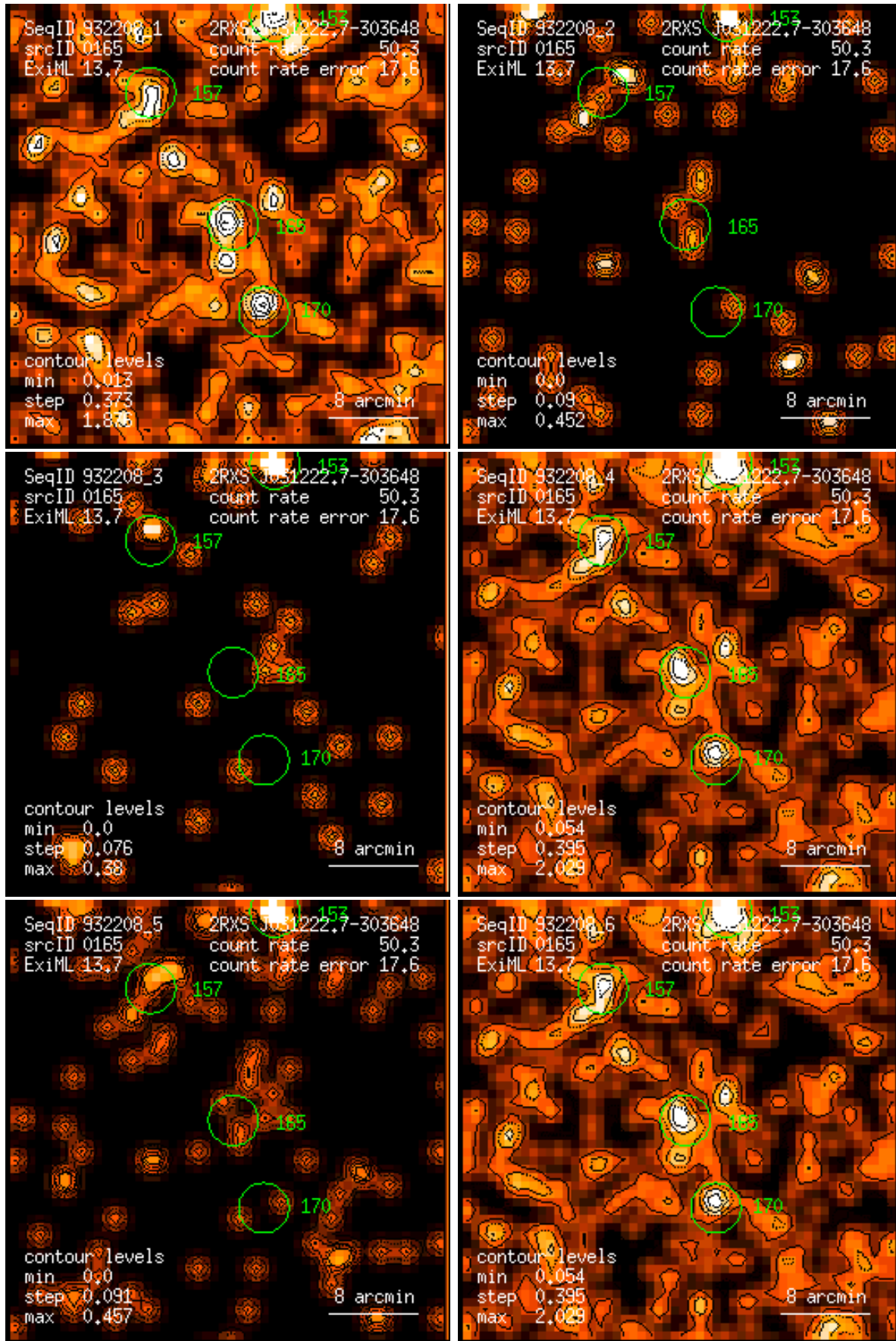
Figure 165: RASS 932208: detection 0165: band rate images, Gaussian filter: (1) PSPC channels 11 – 41, (2) 52 – 90, (3) 91 – 201, (4) 11 – 235, (5) 52 – 201, (6) 11 – 201. Broad band rates in counts/ks. Band rate contour levels in counts/ks/arcmin 2 .
