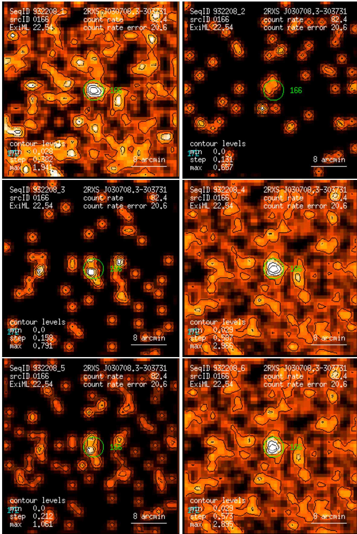
Figure 166: RASS 932208: detection 0166: band rate images, Gaussian filter: (1) PSPC channels 11 – 41, (2) 52 – 90, (3) 91 – 201, (4) 11 – 235, (5) 52 – 201, (6) 11 – 201. Broad band rates in counts/ks. Band rate contour levels in counts/ks/arcmin 2 .
