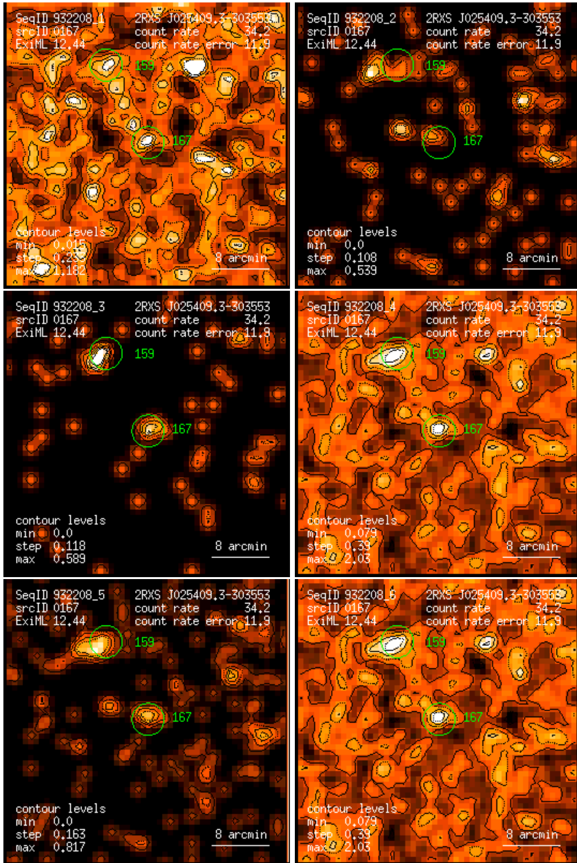
Figure 167: RASS 932208: detection 0167: band rate images, Gaussian filter: (1) PSPC channels 11 – 41, (2) 52 – 90, (3) 91 – 201, (4) 11 – 235, (5) 52 – 201, (6) 11 – 201. Broad band rates in counts/ks. Band rate contour levels in counts/ks/arcmin 2 .
