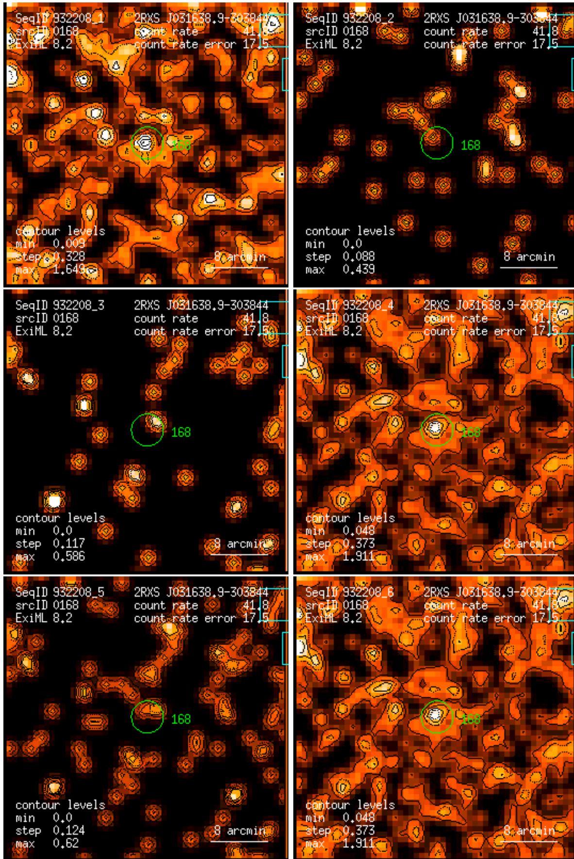
Figure 168: RASS 932208: detection 0168: band rate images, Gaussian filter: (1) PSPC channels 11 – 41, (2) 52 – 90, (3) 91 – 201, (4) 11 – 235, (5) 52 – 201, (6) 11 – 201. Broad band rates in counts/ks. Band rate contour levels in counts/ks/arcmin 2 .
