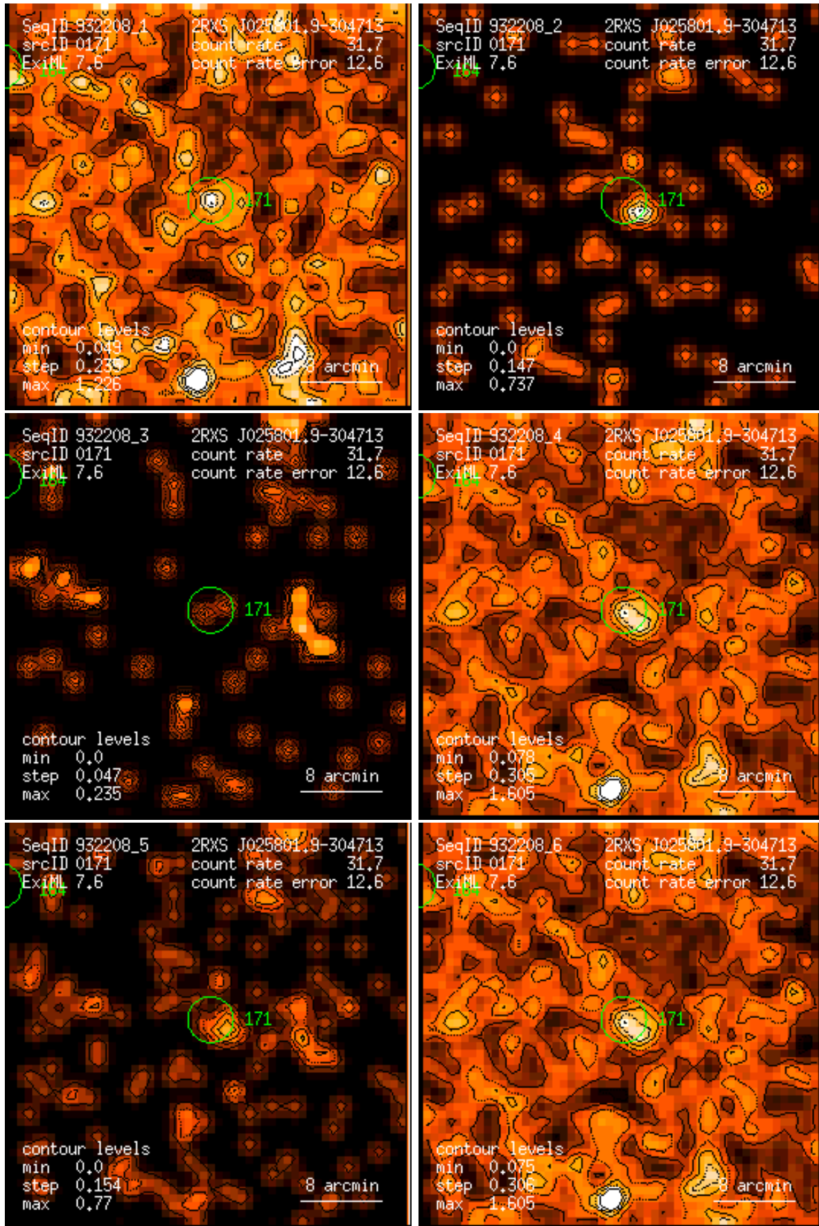
Figure 171: RASS 932208: detection 0171: band rate images, Gaussian filter: (1) PSPC channels 11 – 41, (2) 52 – 90, (3) 91 – 201, (4) 11 – 235, (5) 52 – 201, (6) 11 – 201. Broad band rates in counts/ks. Band rate contour levels in counts/ks/arcmin 2 .
