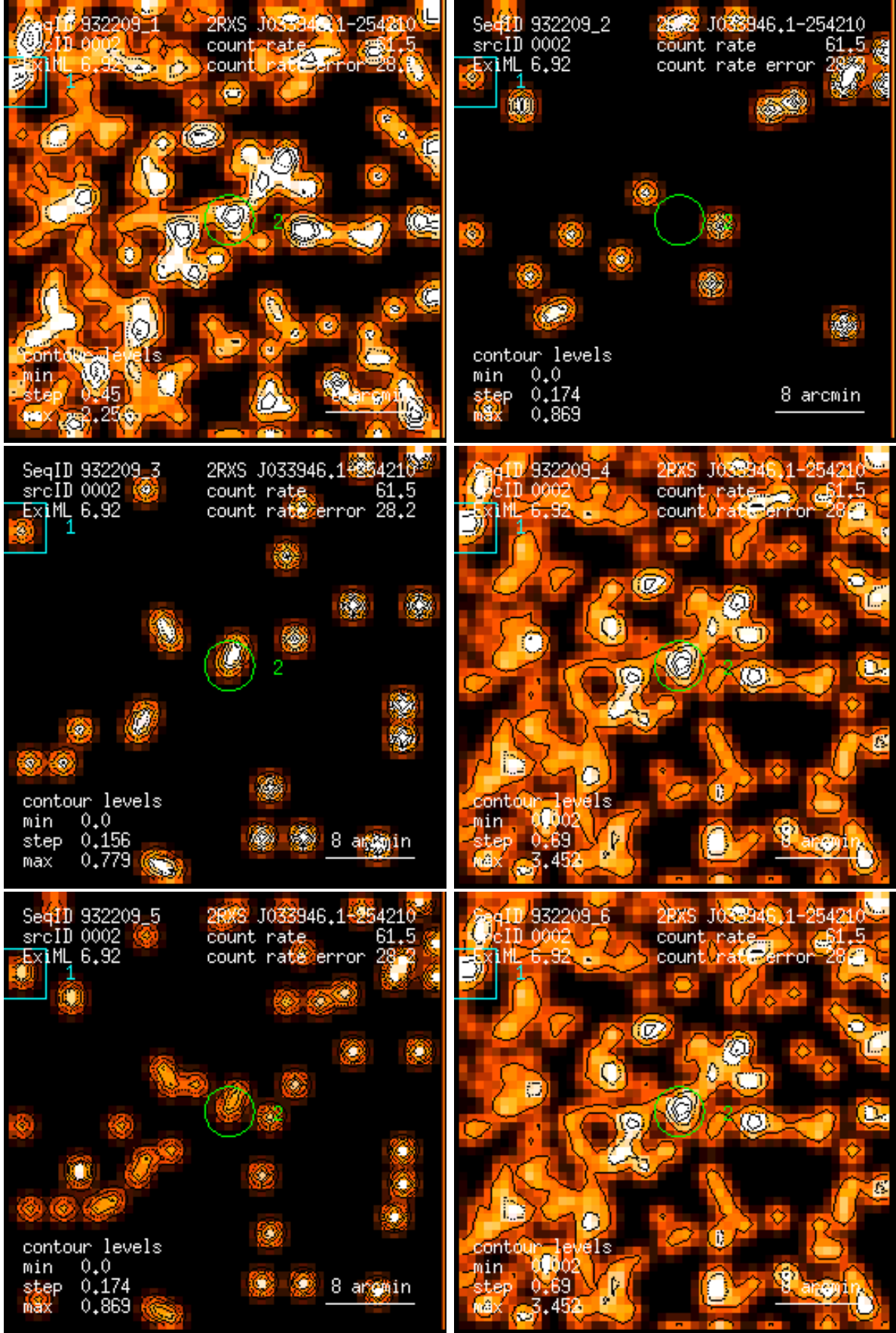
Figure 2: RASS 932209: detection 0002: band rate images, Gaussian filter: (1) PSPC channels 11 – 41, (2) 52 – 90, (3) 91 – 201, (4) 11 – 235, (5) 52 – 201, (6) 11 – 201. Broad band rates in counts/ks. Band rate contour levels in counts/ks/arcmin 2 .
